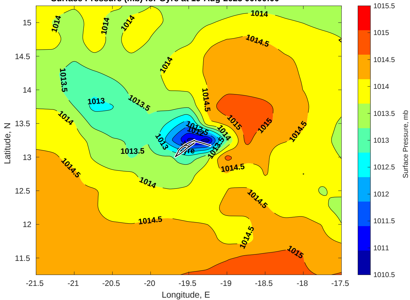
Surface Pressure (mb) for Gyre at 19-Aug-2025 00:00:00
