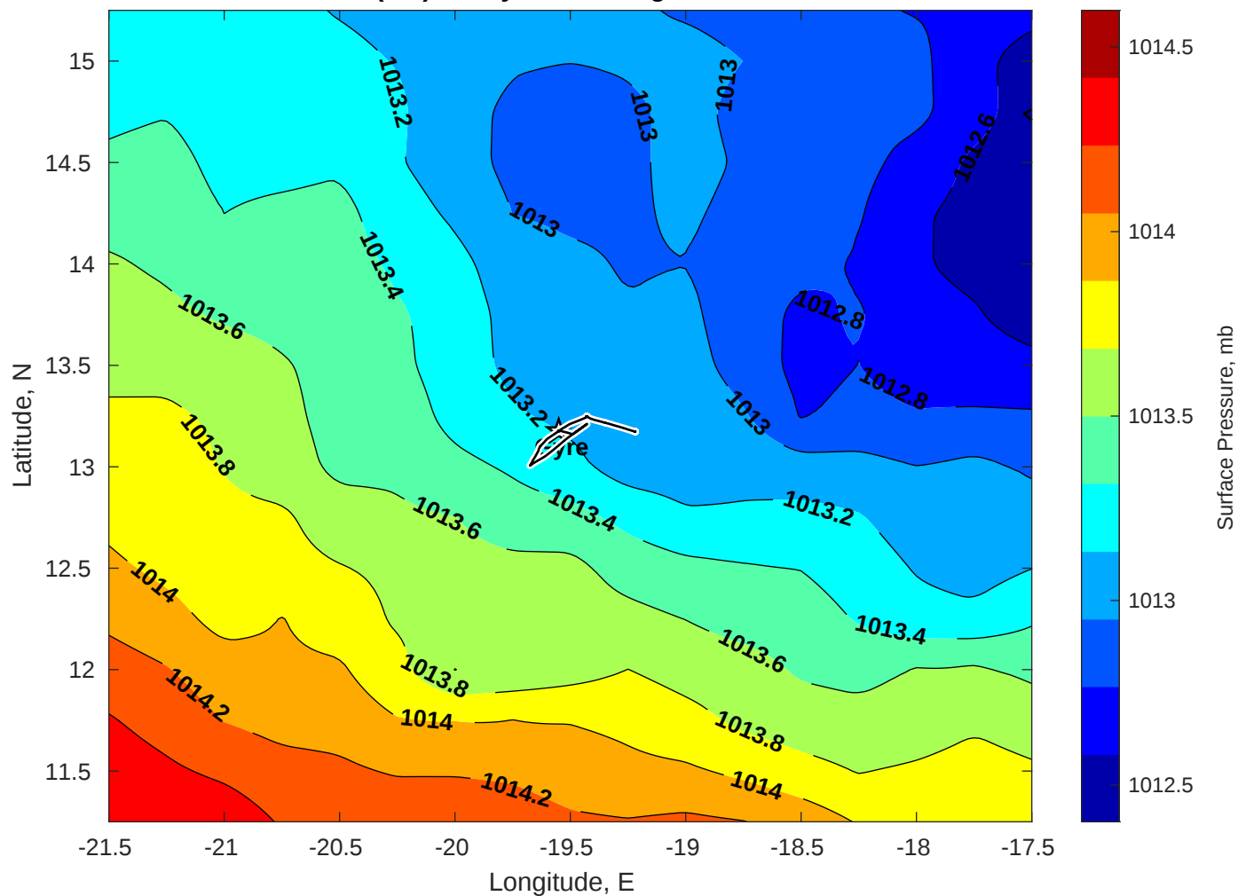
Surface Pressure (mb) for Gyre at 21-Aug-2025 00:00:00
