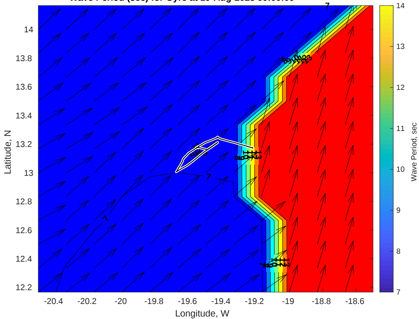
Wave Period (sec) for Gyre at 19-Aug-2025 09:00:00
