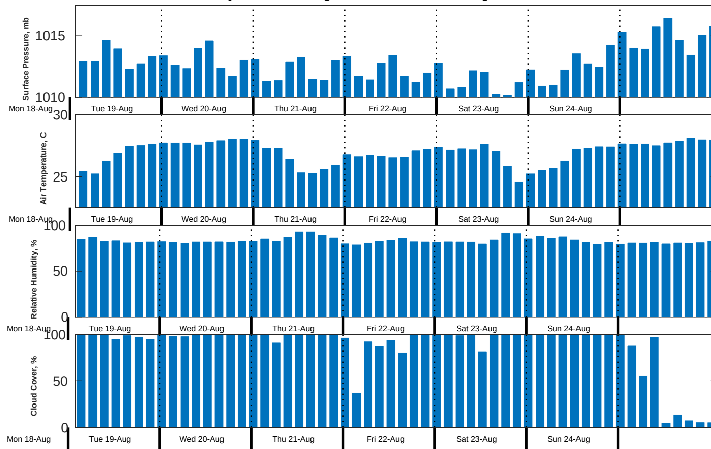
Met Forecast for Gyre from 18-Aug-2025 23:00:00 to 25-Aug-2025 23:00:00
