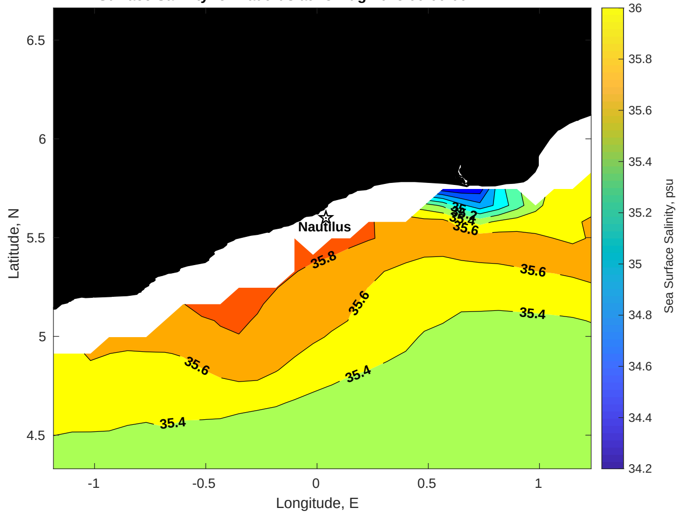
Surface Salinity for Nautilus at 18-Aug-2025 00:00:00
