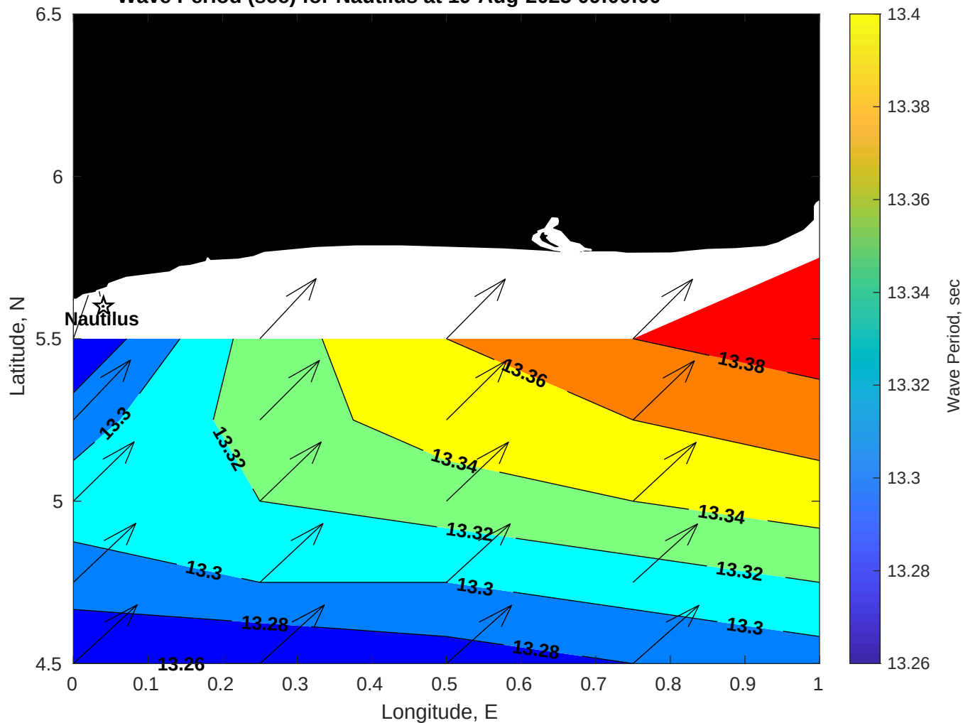
Wave Period (sec) for Nautilus at 19-Aug-2025 09:00:00
