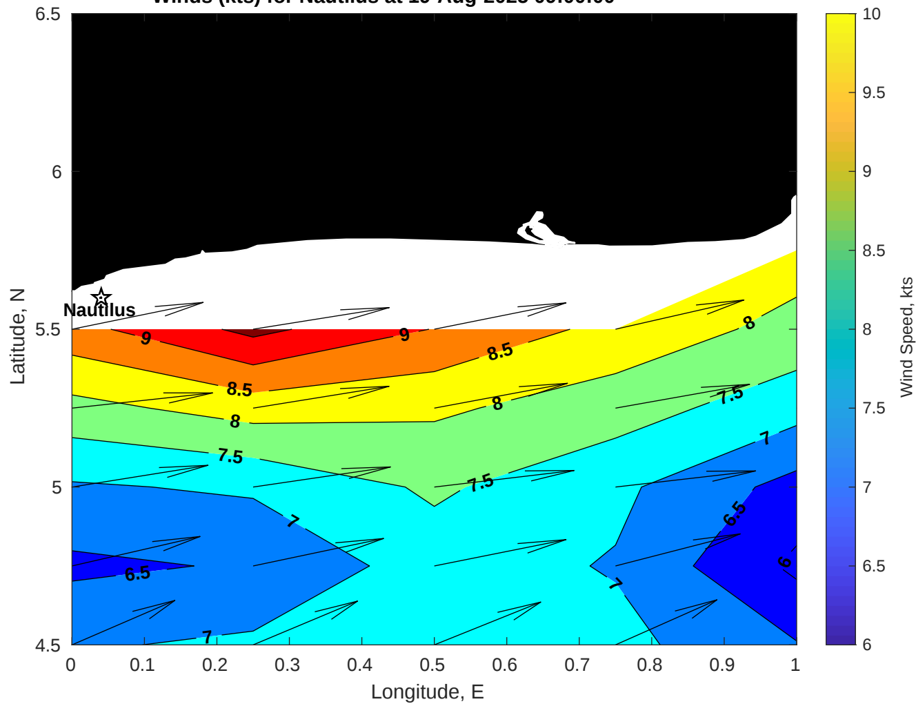
Winds (kts) for Nautilus at 19-Aug-2025 09:00:00
