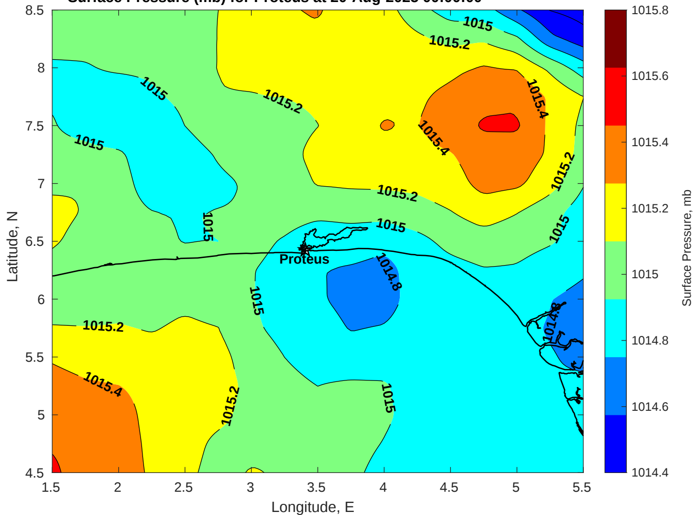
Surface Pressure (mb) for Proteus at 20-Aug-2025 00:00:00
