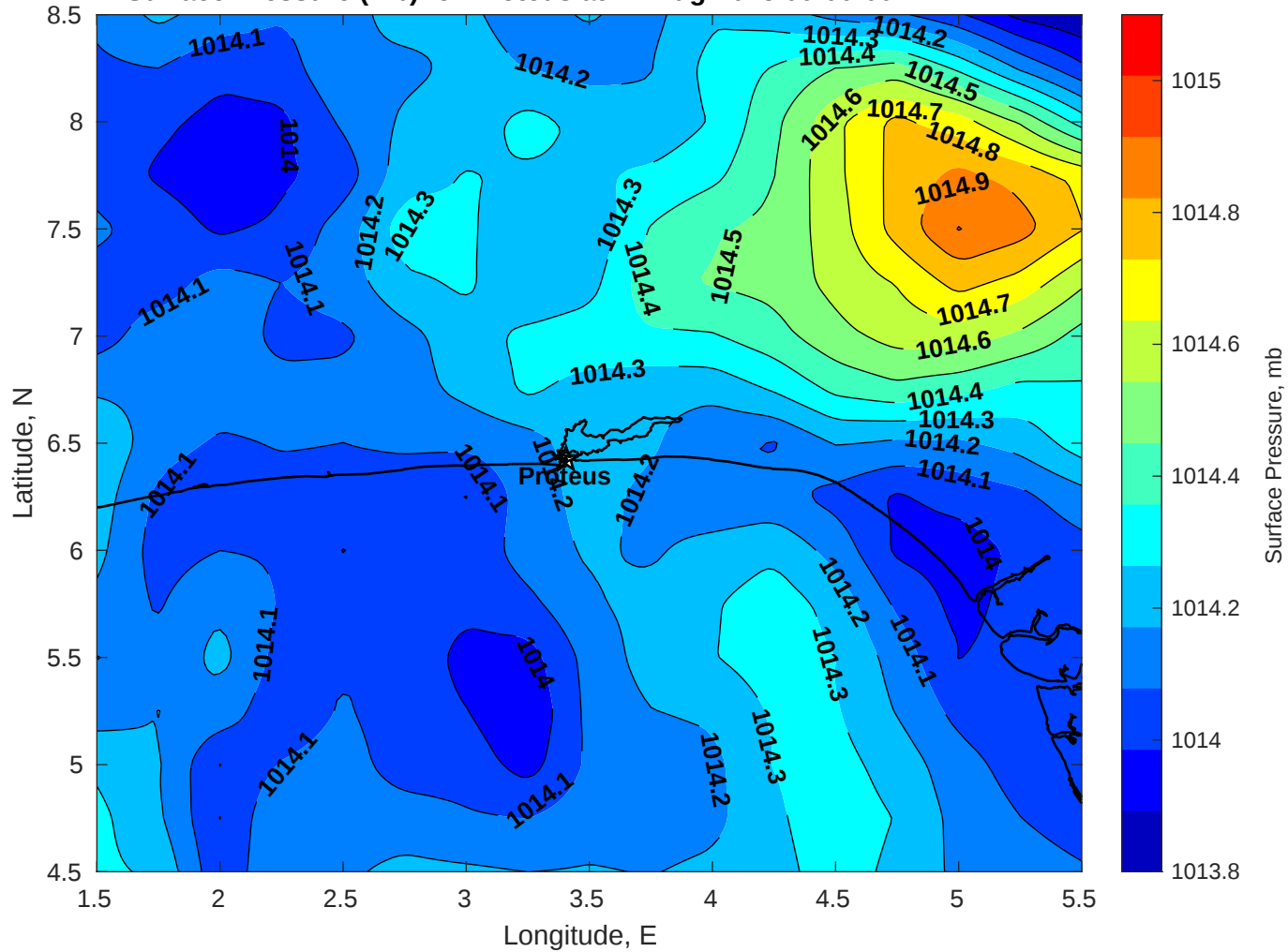
Surface Pressure (mb) for Proteus at 21-Aug-2025 00:00:00
