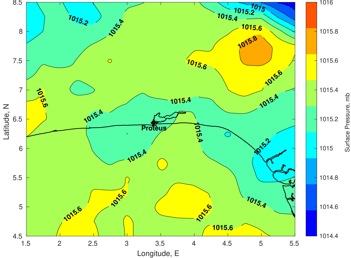
Surface Pressure (mb) for Proteus at 19-Aug-2025 00:00:00
