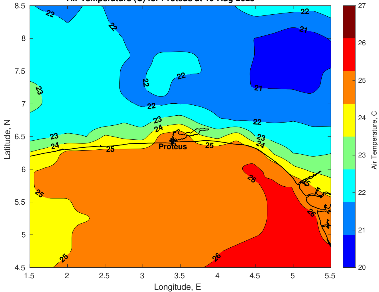
Air Temperature (C) for Proteus at 19-Aug-2025
