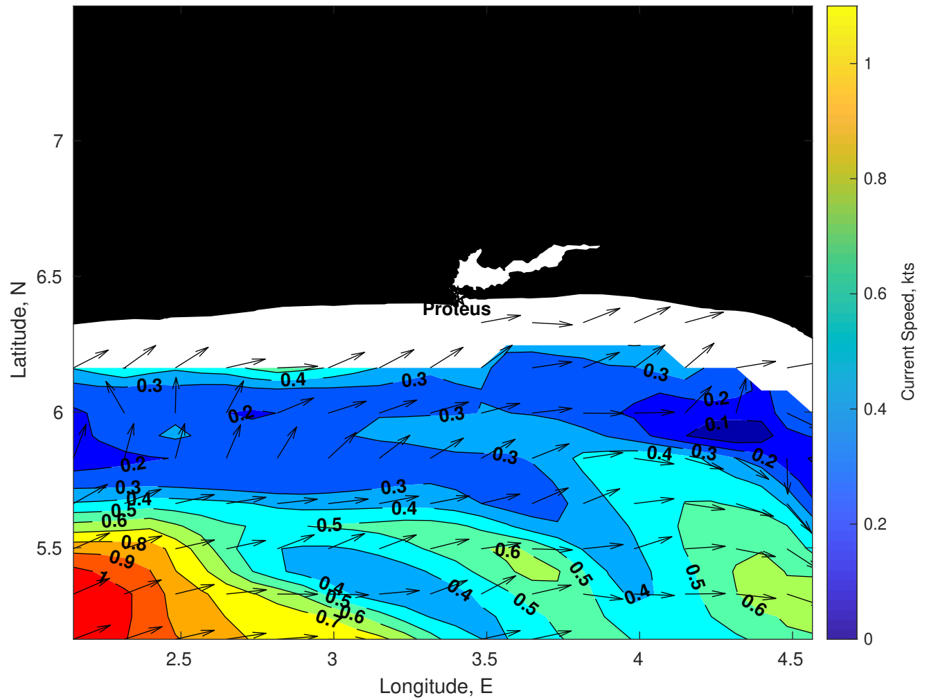
Surface Currents for Proteus at 18-Aug-2025 00:00:00
