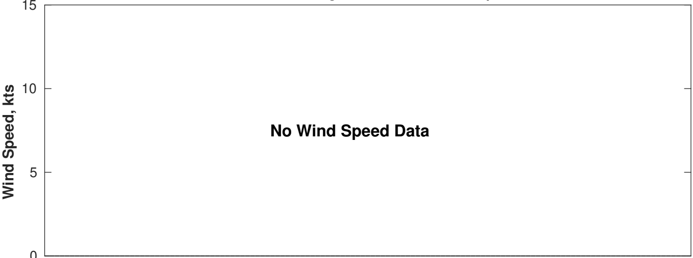
Wind & Wave Forecast for Proteus from 19-Aug-2025 01:00:00 to 04-Sep-2025 01:00:00
