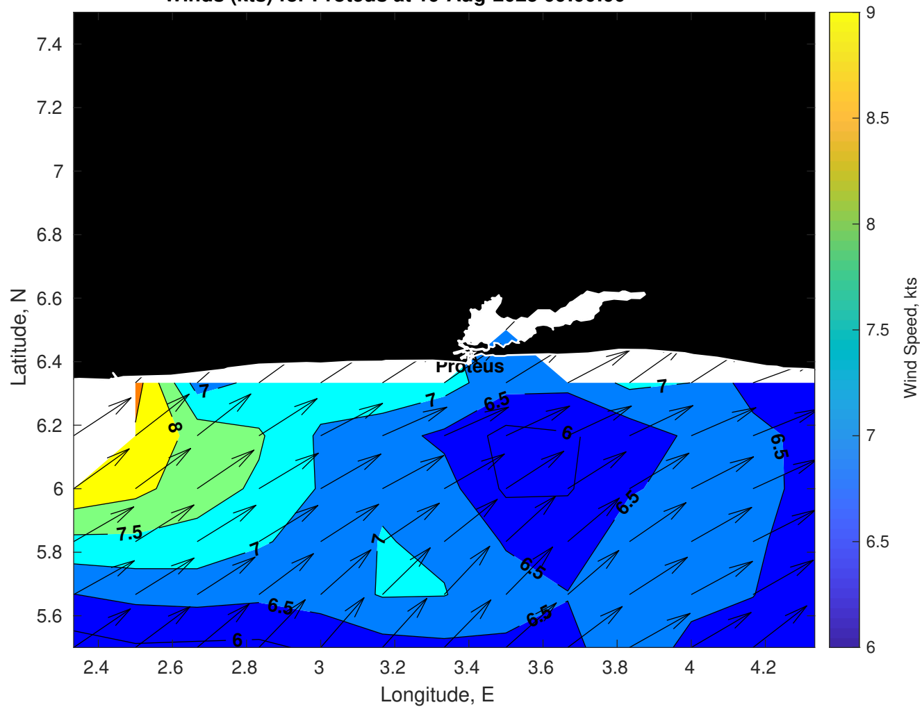
Winds (kts) for Proteus at 19-Aug-2025 09:00:00
