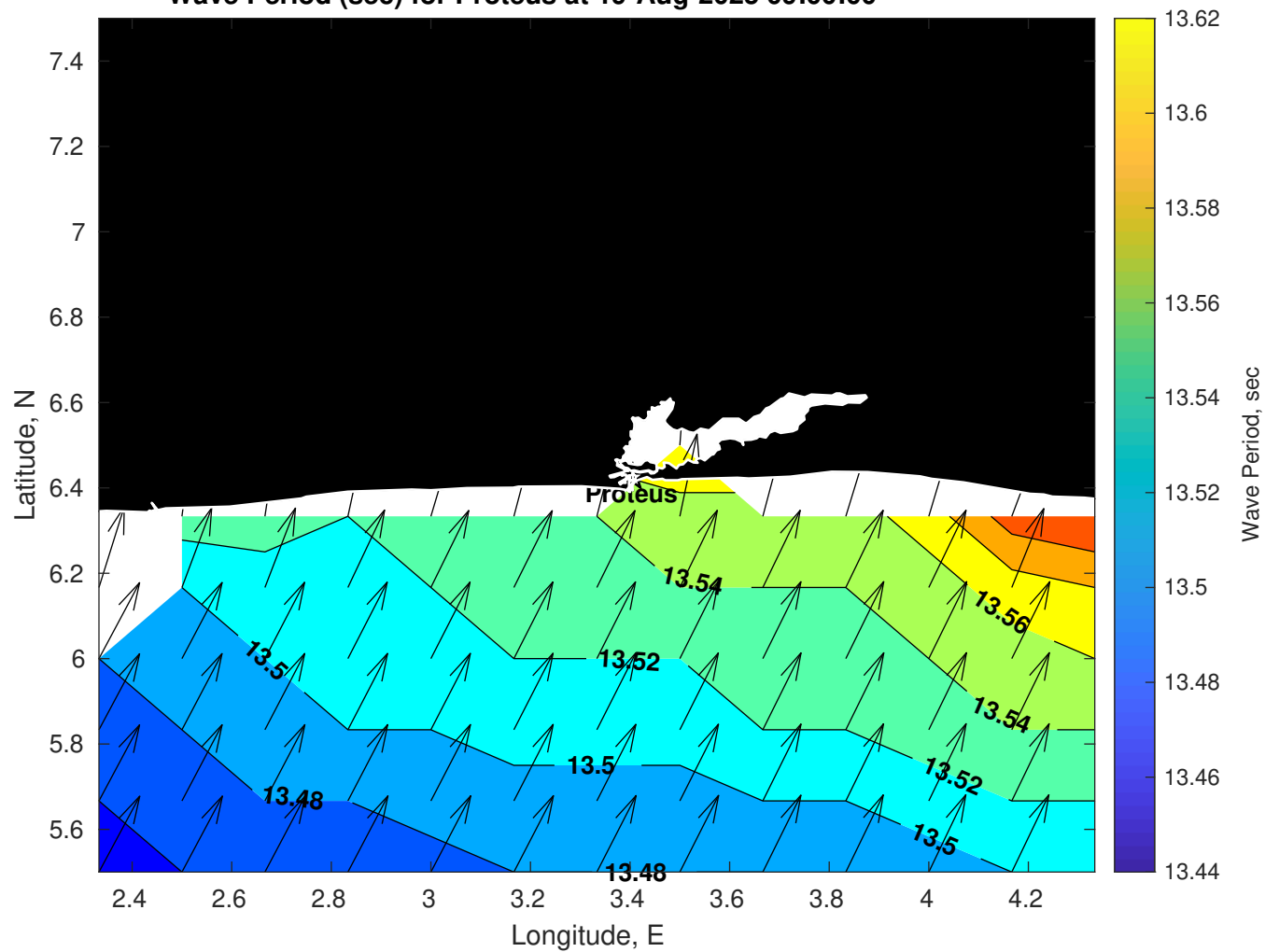
Wave Period (sec) for Proteus at 19-Aug-2025 09:00:00
