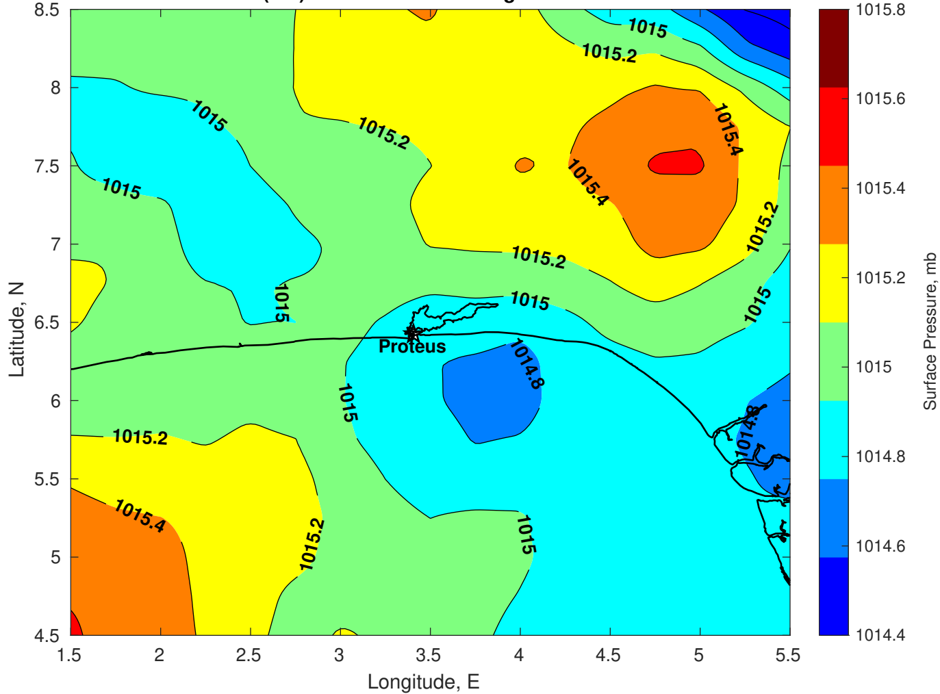
Surface Pressure (mb) for Proteus at 20-Aug-2025 00:00:00
