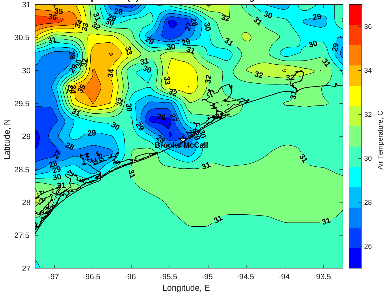
Air Temperature (C) for Brooks McCall at 20-Aug-2025
