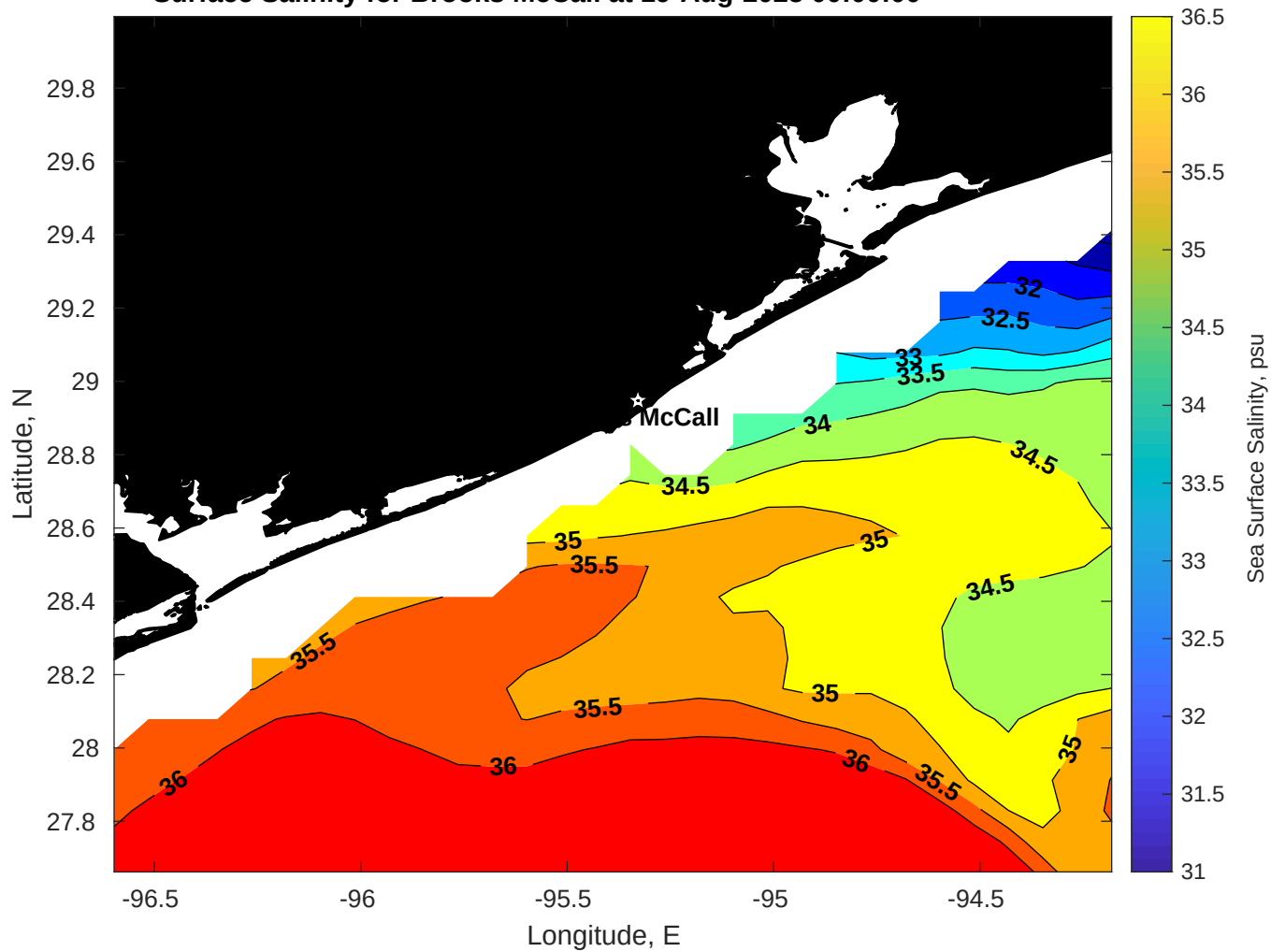
Surface Salinity for Brooks McCall at 19-Aug-2025 00:00:00
