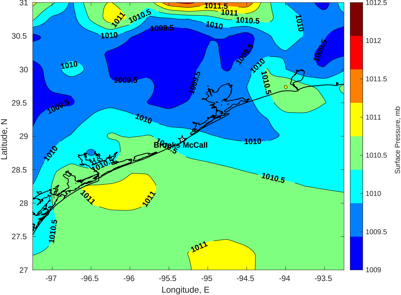
Surface Pressure (mb) for Brooks McCall at 21-Aug-2025 00:00:00
