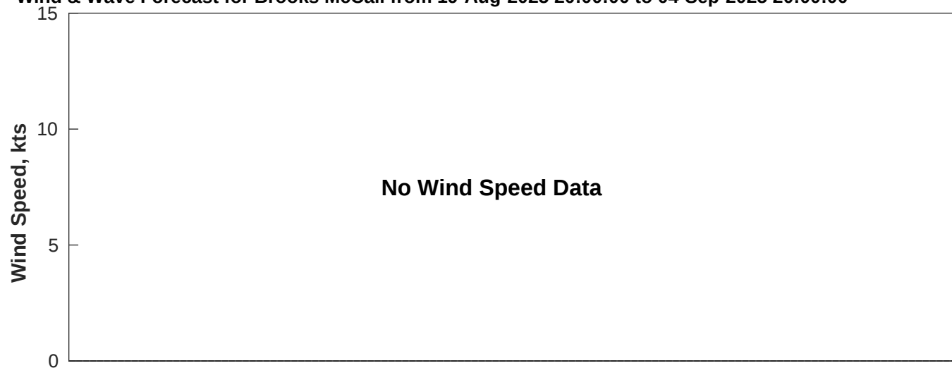
Wind & Wave Forecast for Brooks McCall from 19-Aug-2025 20:00:00 to 04-Sep-2025 20:00:00
