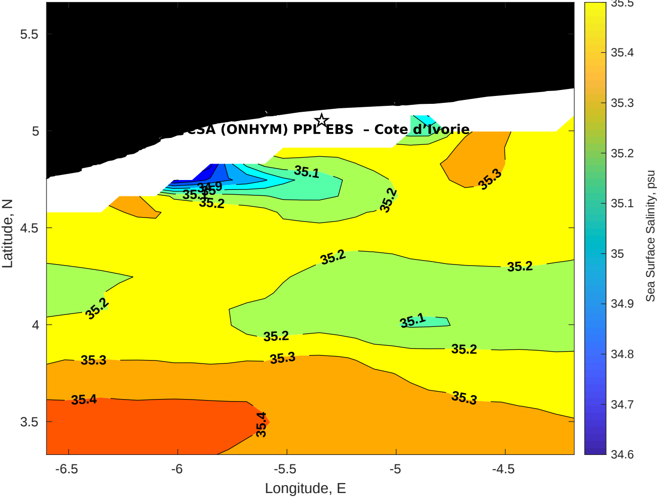
Surface Salinity for CSA (ONHYM) PPL EBS - Cote d'Ivoire at 19-Aug-2025 00:00:00
