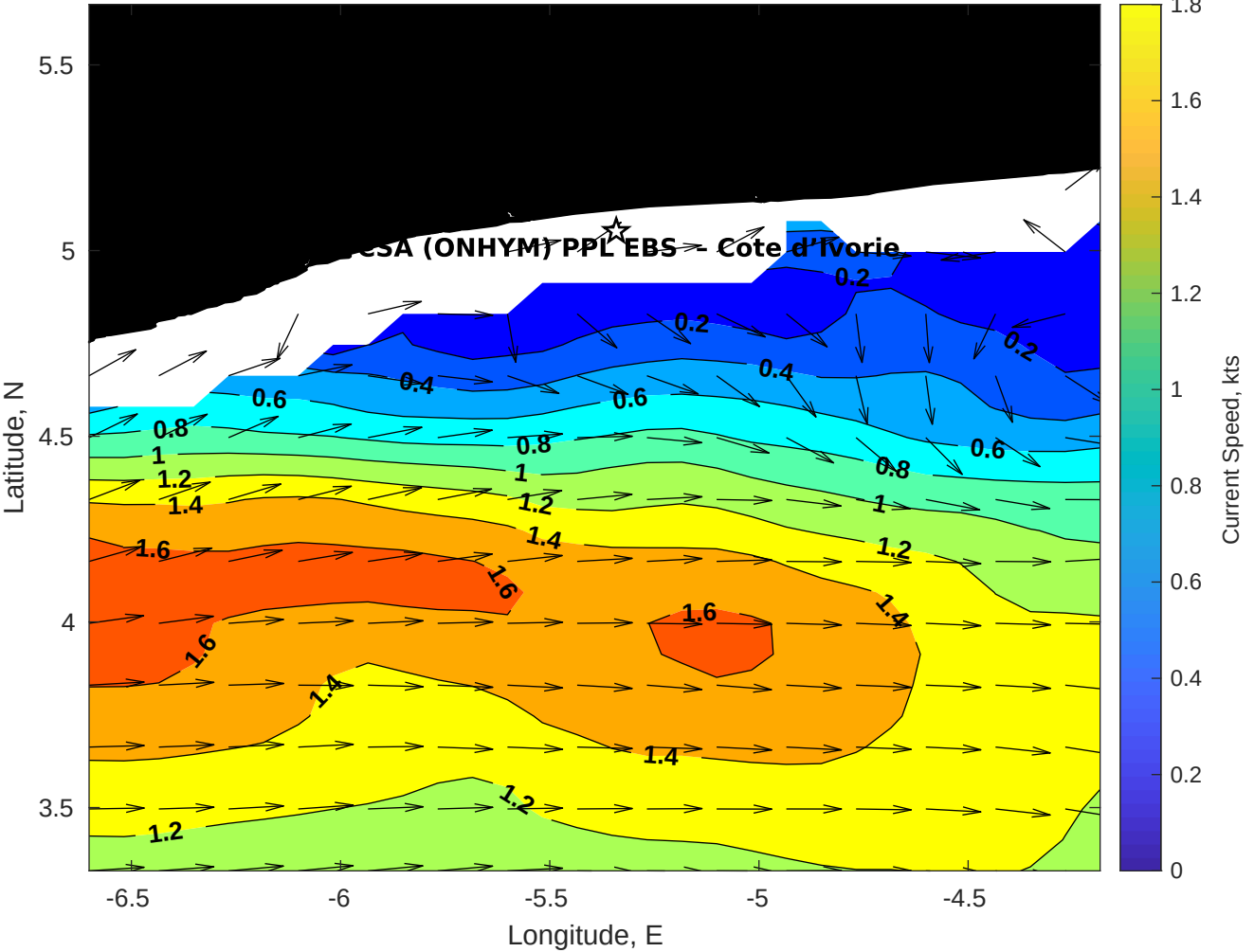
Surface Currents for CSA (ONHYM) PPL EBS - Cote d'Ivoire at 19-Aug-2025 00:00:00
