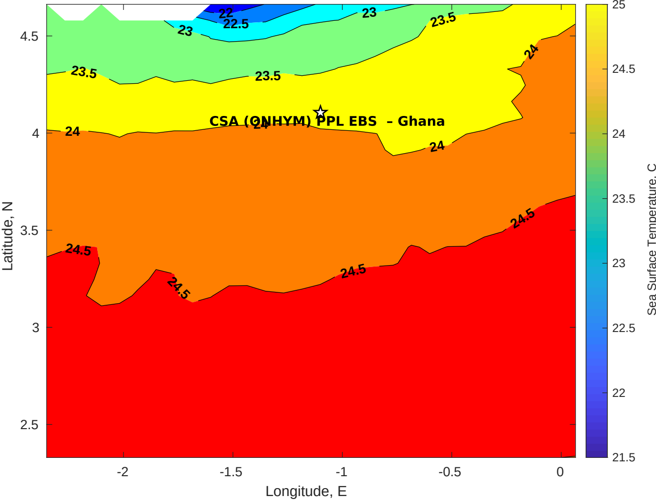
SST for CSA (ONHYM) PPL EBS - Ghana at 19-Aug-2025 00:00:00
