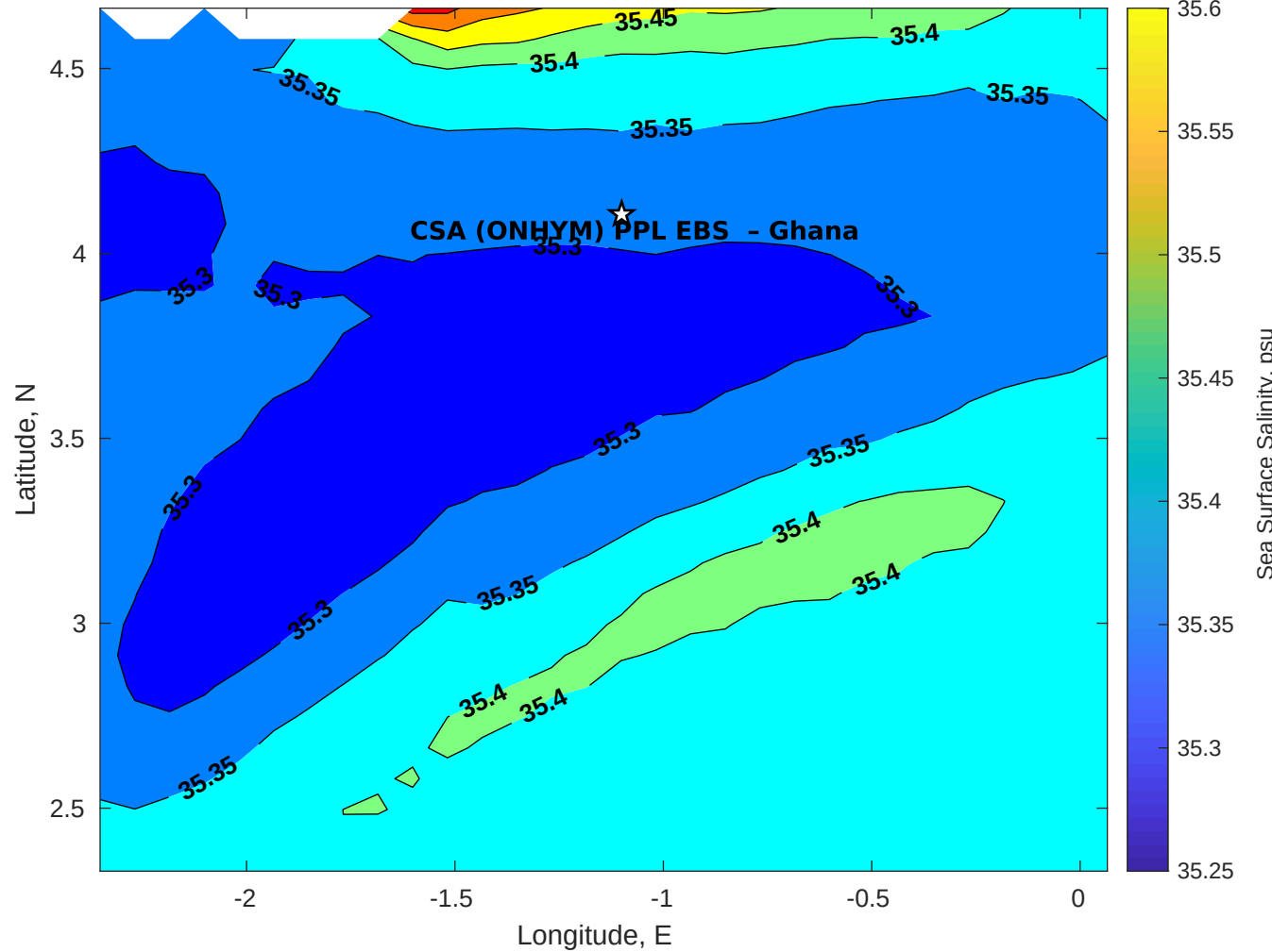
Surface Salinity for CSA (ONHYM) PPL EBS - Ghana at 19-Aug-2025 00:00:00
