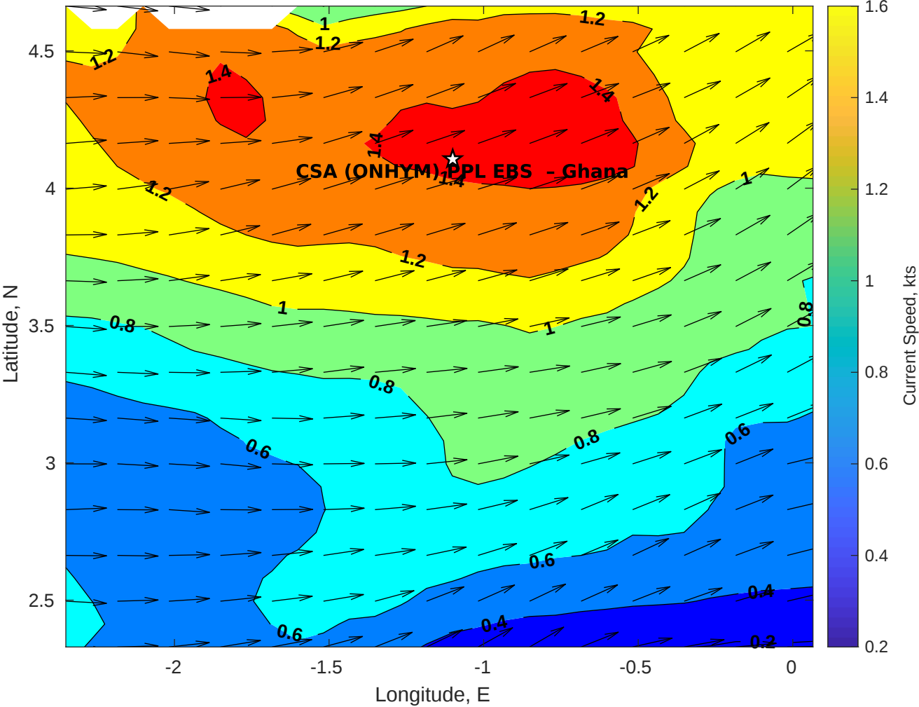
Surface Currents for CSA (ONHYM) PPL EBS - Ghana at 19-Aug-2025 00:00:00
