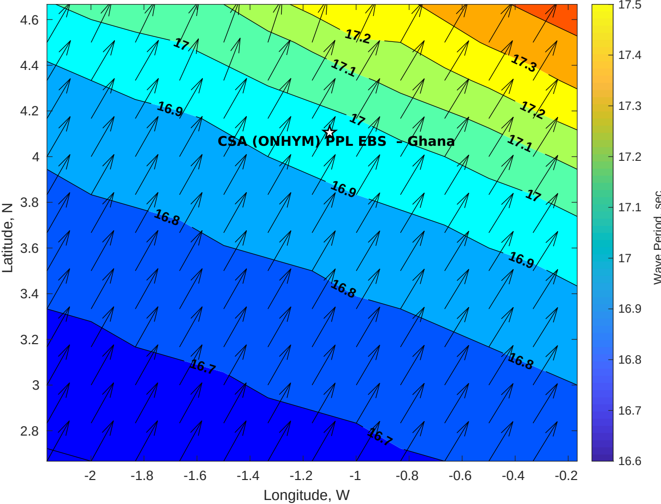
Wave Period (sec) for CSA (ONHYM) PPL EBS - Ghana at 20-Aug-2025 09:00:00
