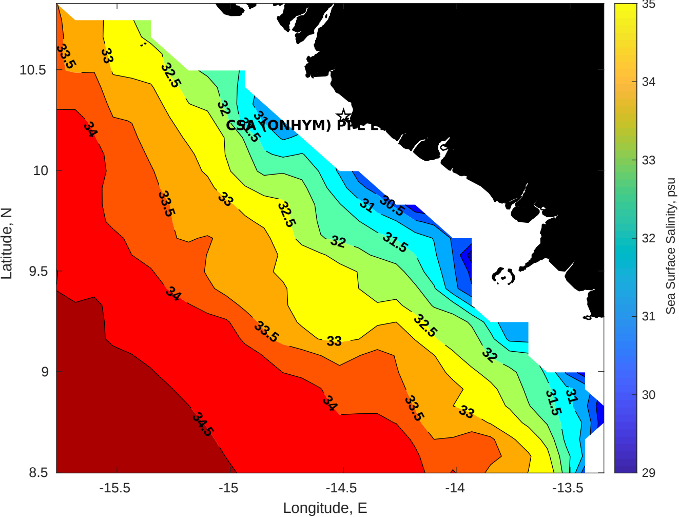
Surface Salinity for CSA (ONHYM) PPL EBS - Guinea at 19-Aug-2025 00:00:00
