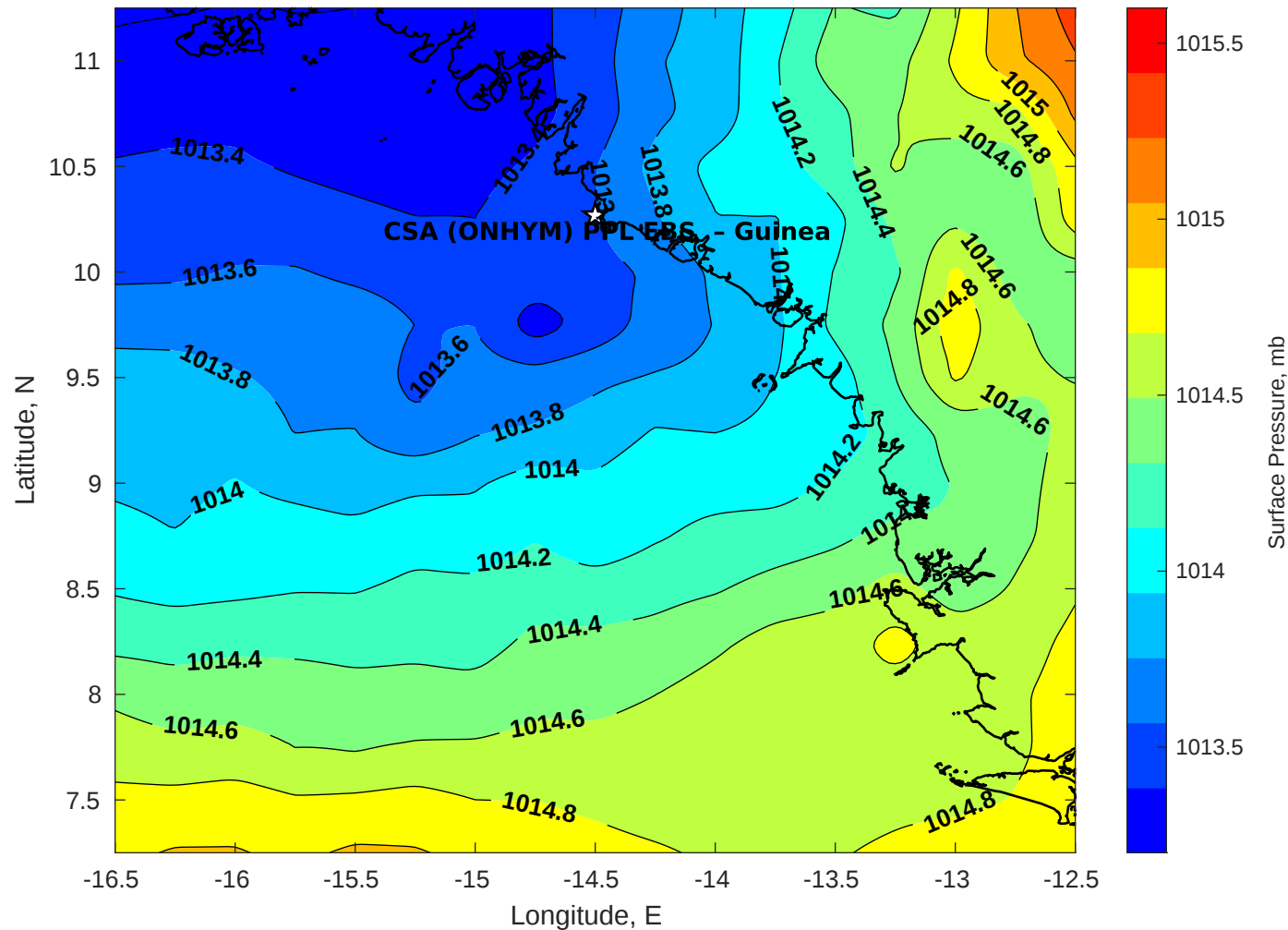
Surface Pressure (mb) for CSA (ONHYM) PPL EBS - Guinea at 21-Aug-2025 00:00:00
