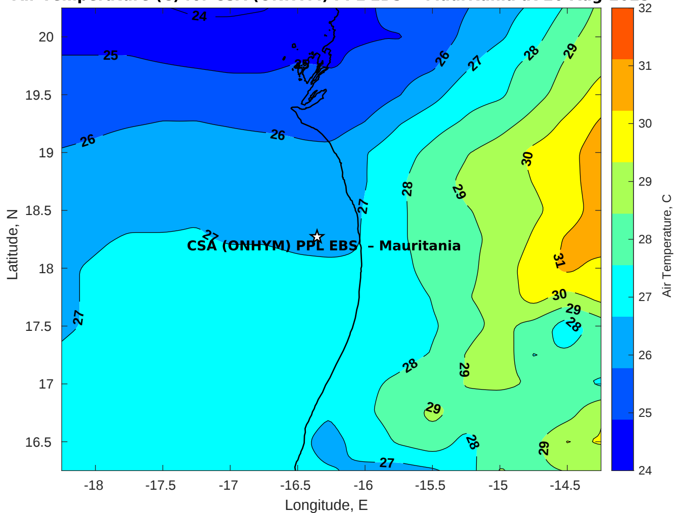
Air Temperature (C) for CSA (ONHYM) PPL EBS - Mauritania at 20-Aug-2025
