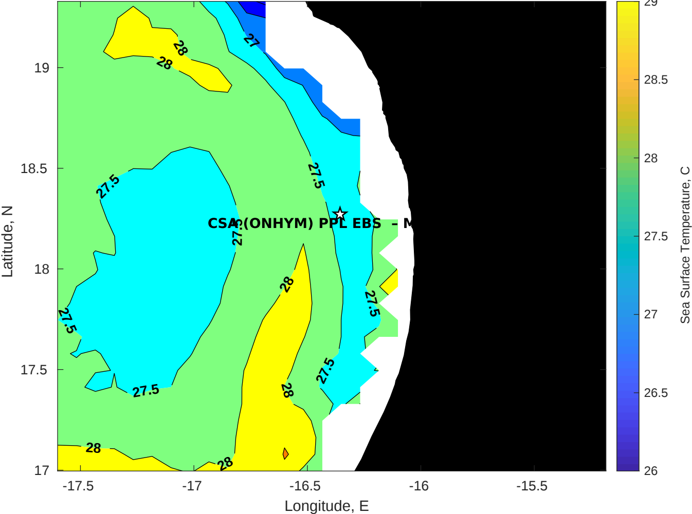
SST for CSA (ONHYM) PPL EBS - Mauritania at 19-Aug-2025 00:00:00
