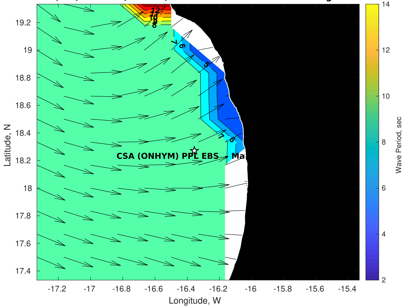
Wave Period (sec) for CSA (ONHYM) PPL EBS - Mauritania at 20-Aug-2025 09:00:00
