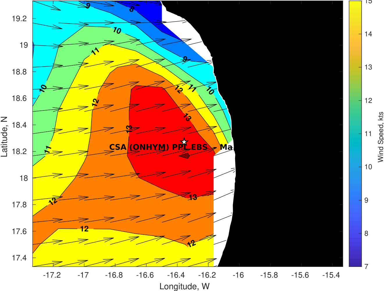
Winds (kts) for CSA (ONHYM) PPL EBS - Mauritania at 20-Aug-2025 09:00:00
