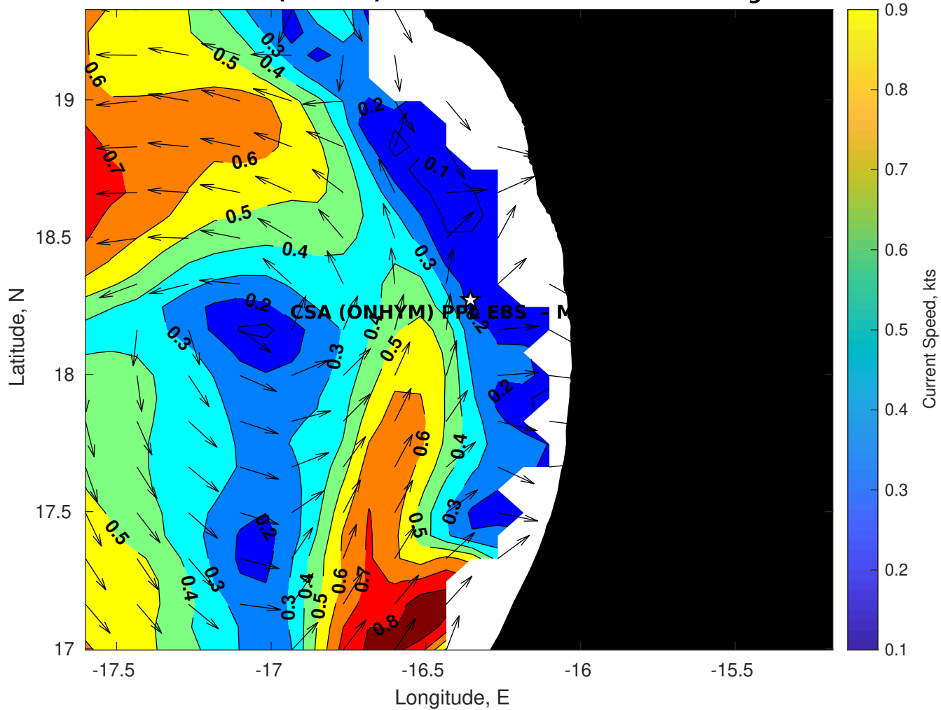
Surface Currents for CSA (ONHYM) PPL EBS - Mauritania at 19-Aug-2025 00:00:00
