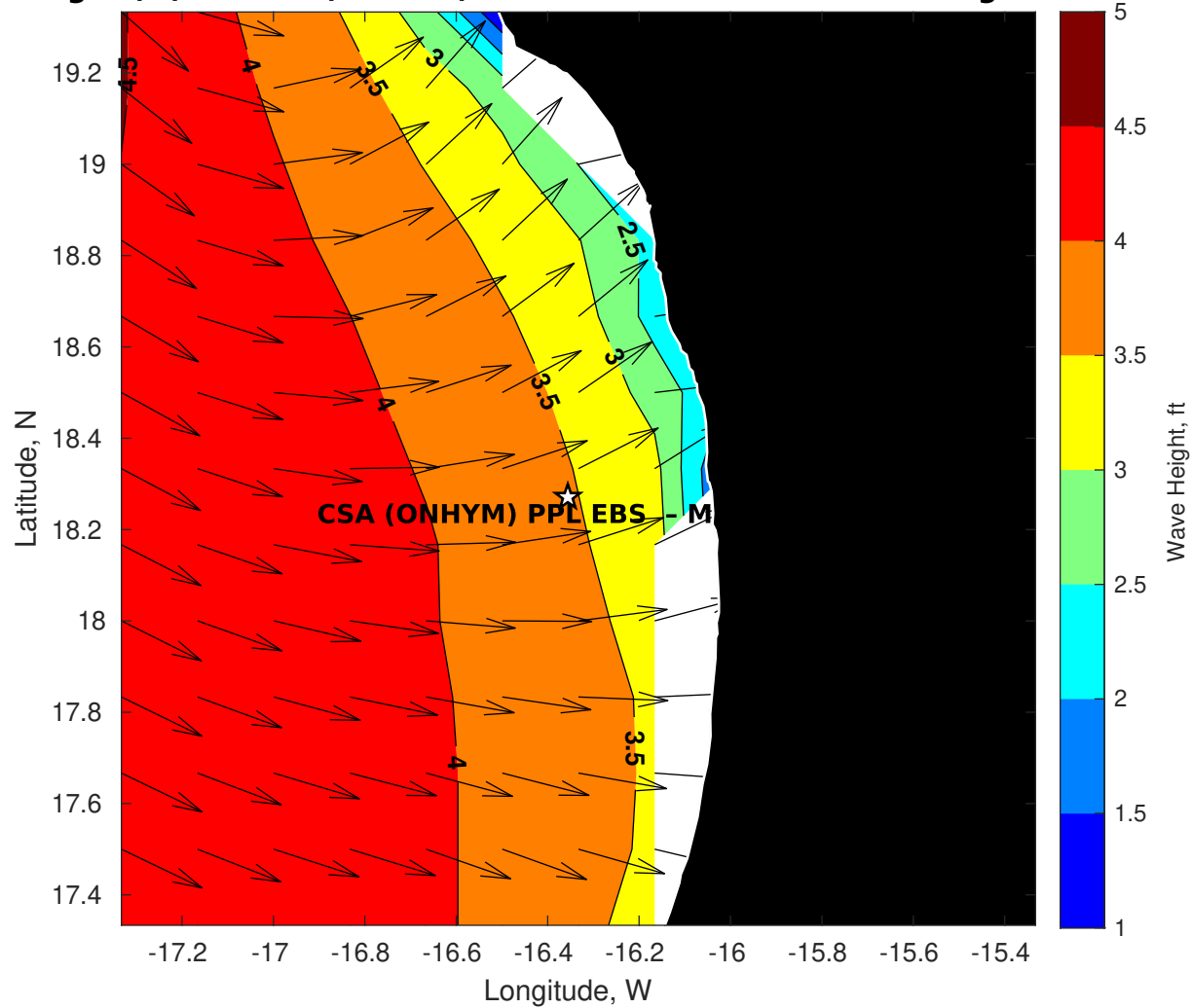
Wave Height (ft) for CSA (ONHYM) PPL EBS - Mauritania at 20-Aug-2025 09:00:00
