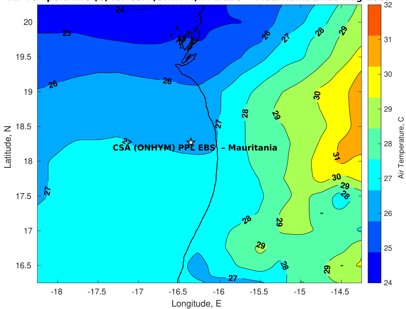
Air Temperature (C) for CSA (ONHYM) PPL EBS - Mauritania at 20-Aug-2025
