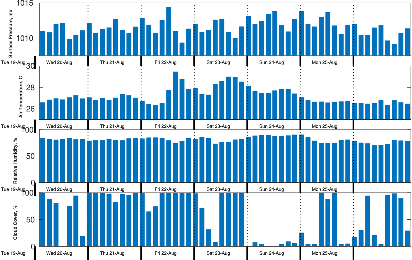
Met Forecast for CSA (ONHYM) PPL EBS - Mauritania from 20-Aug-2025 00:00:00 to 27-Aug-2025 00:00:00
