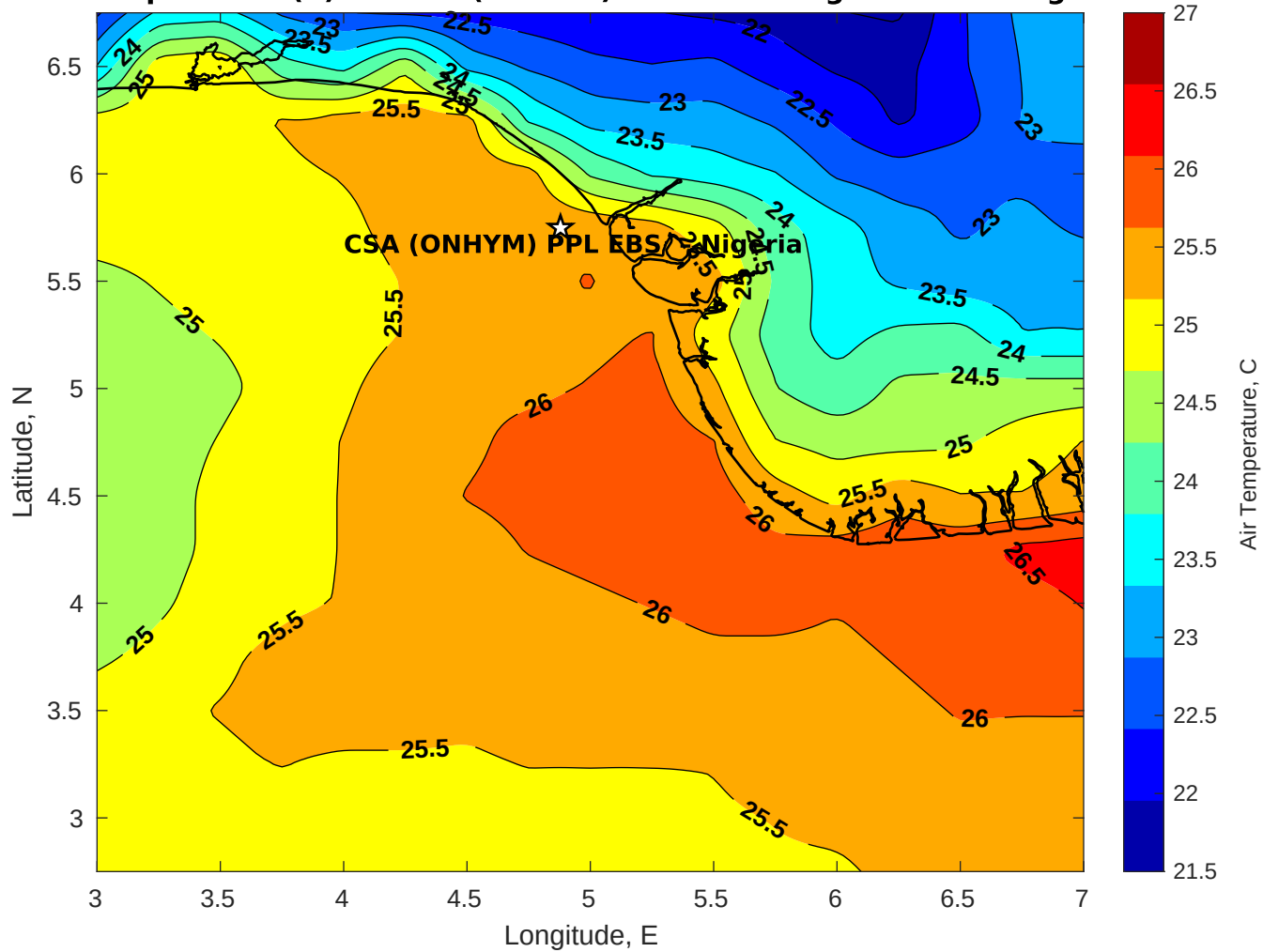
Air Temperature (C) for CSA (ONHYM) PPL EBS - Nigeria at 20-Aug-2025
