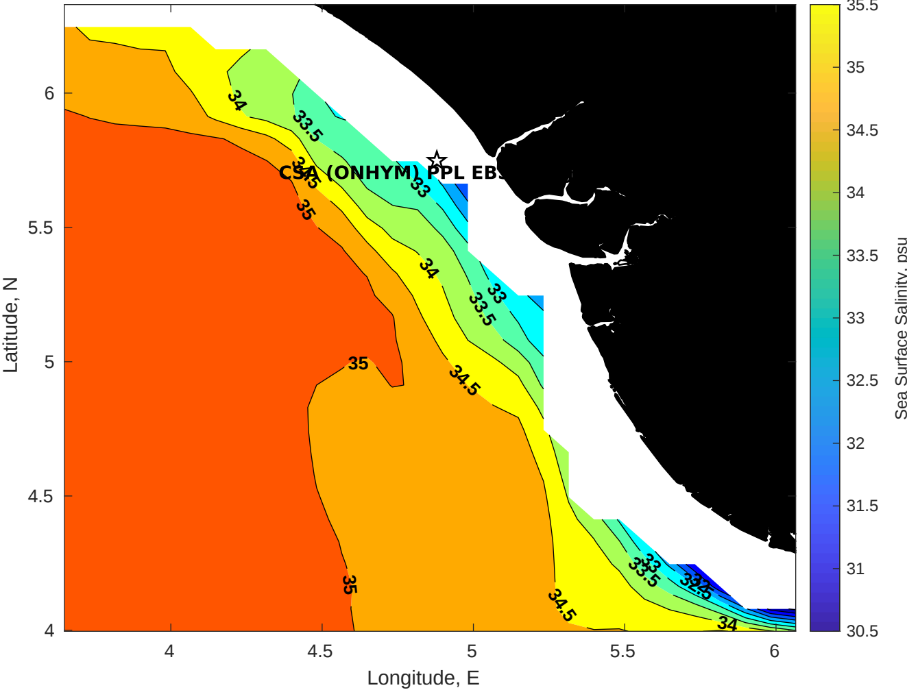
Surface Salinity for CSA (ONHYM) PPL EBS - Nigeria at 19-Aug-2025 00:00:00
