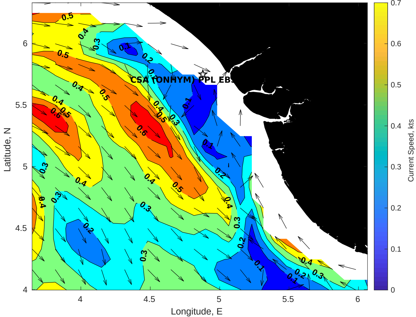
Surface Currents for CSA (ONHYM) PPL EBS - Nigeria at 19-Aug-2025 00:00:00
