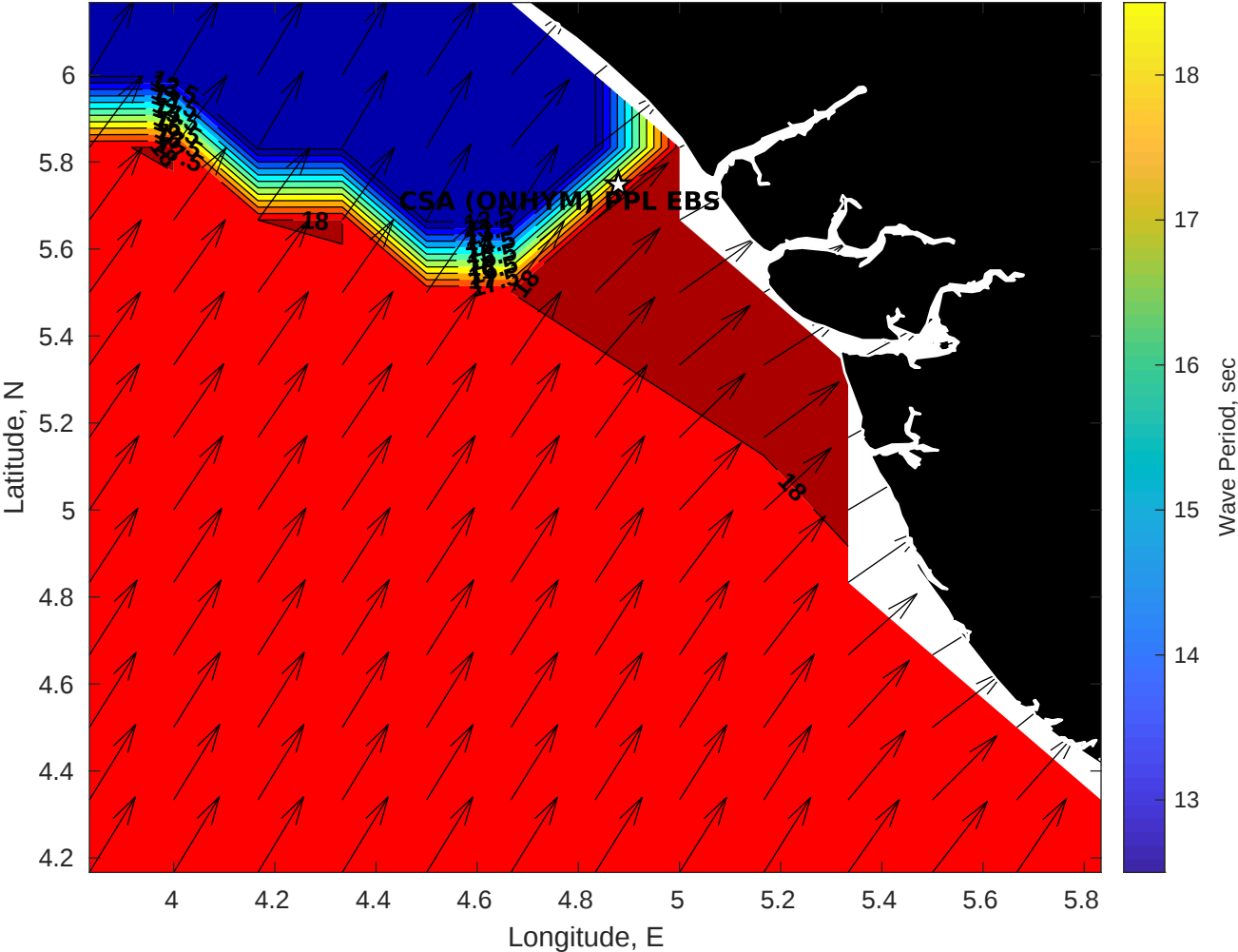
Wave Period (sec) for CSA (ONHYM) PPL EBS - Nigeria at 20-Aug-2025 09:00:00
