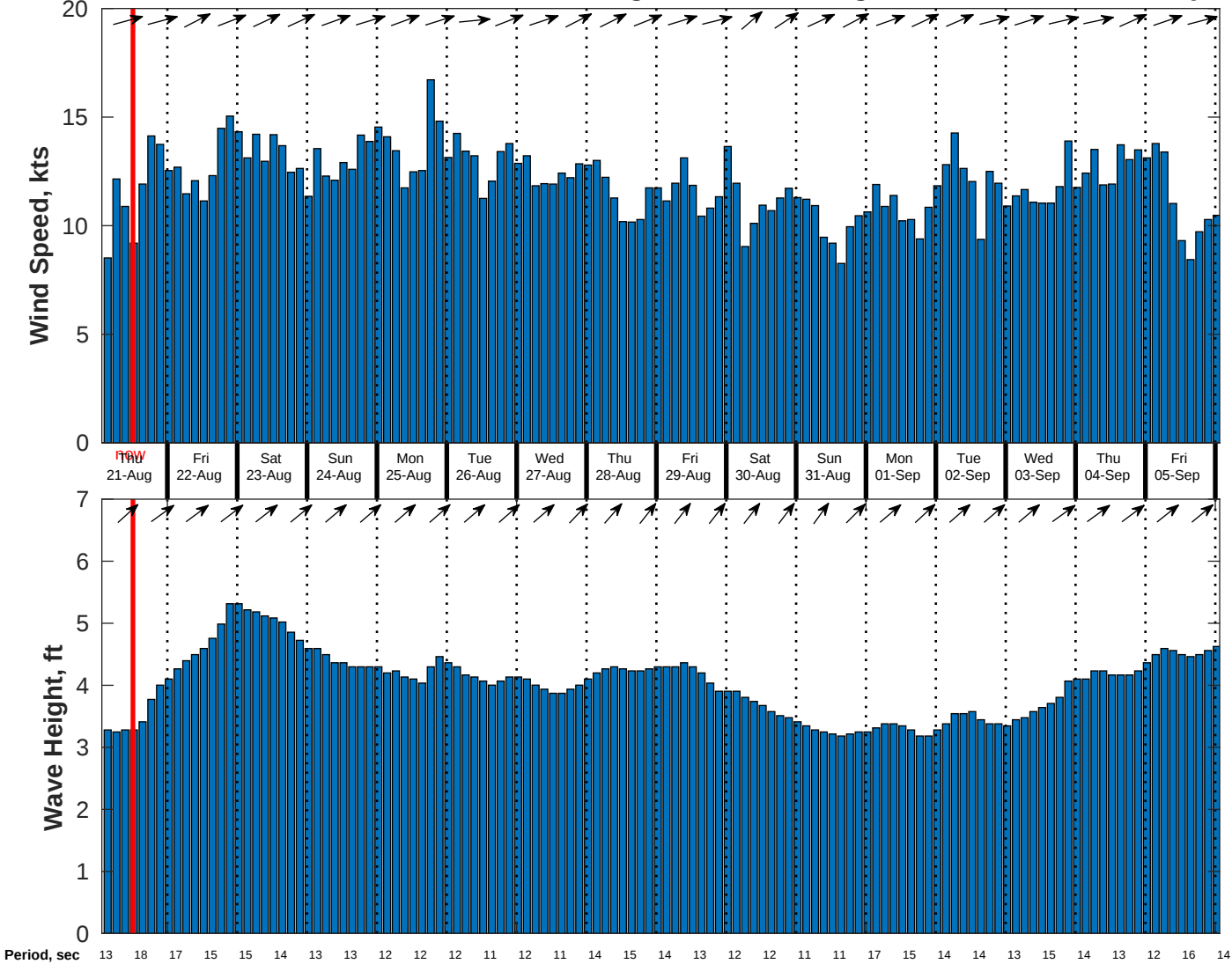
Wind & Wave Forecast for CSA (ONHYM) PPL EBS - Nigeria from 20-Aug-2025 02:00:00 to 05-Sep-2025 02:00:00
