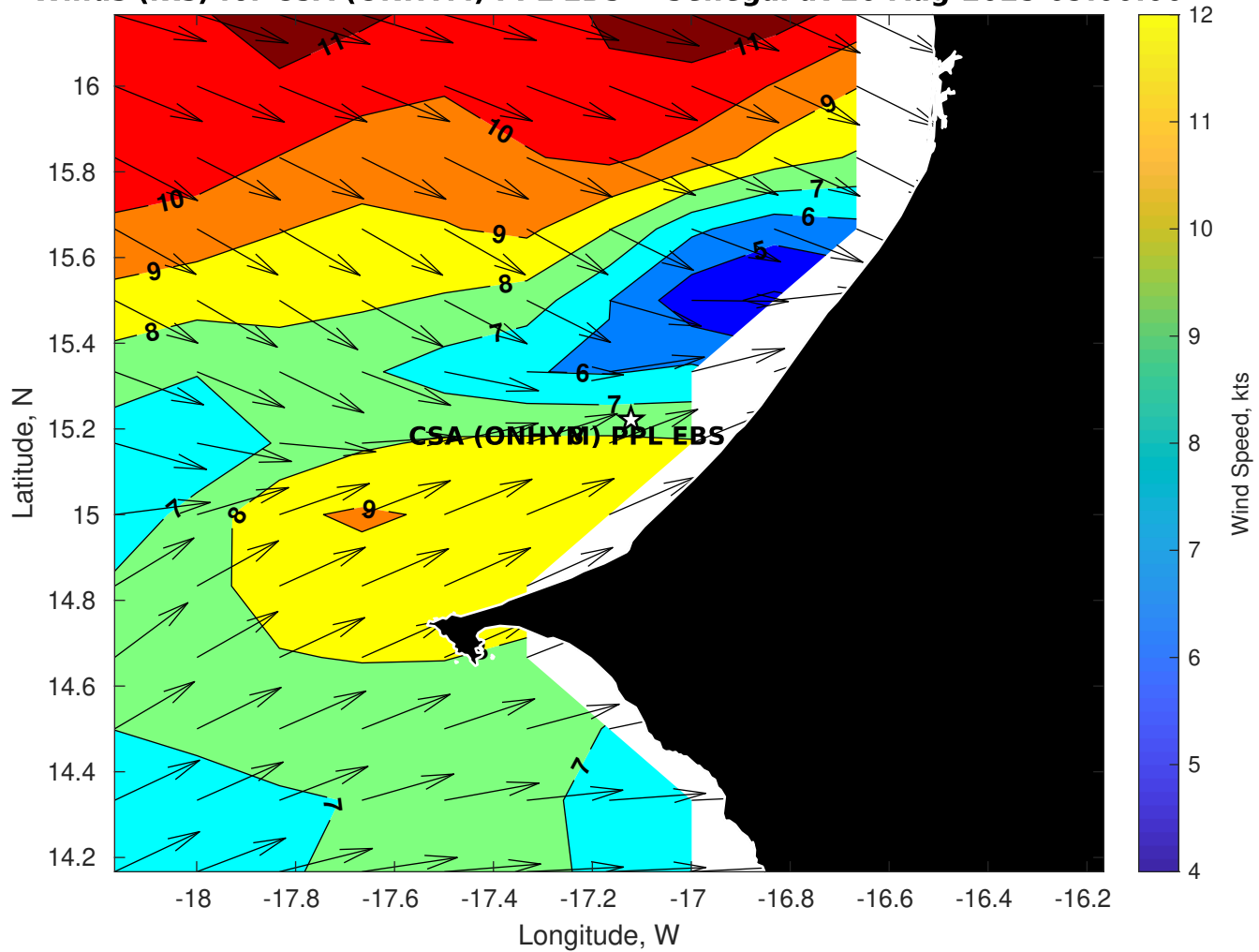
Winds (kts) for CSA (ONHYM) PPL EBS - Senegal at 20-Aug-2025 09:00:00
