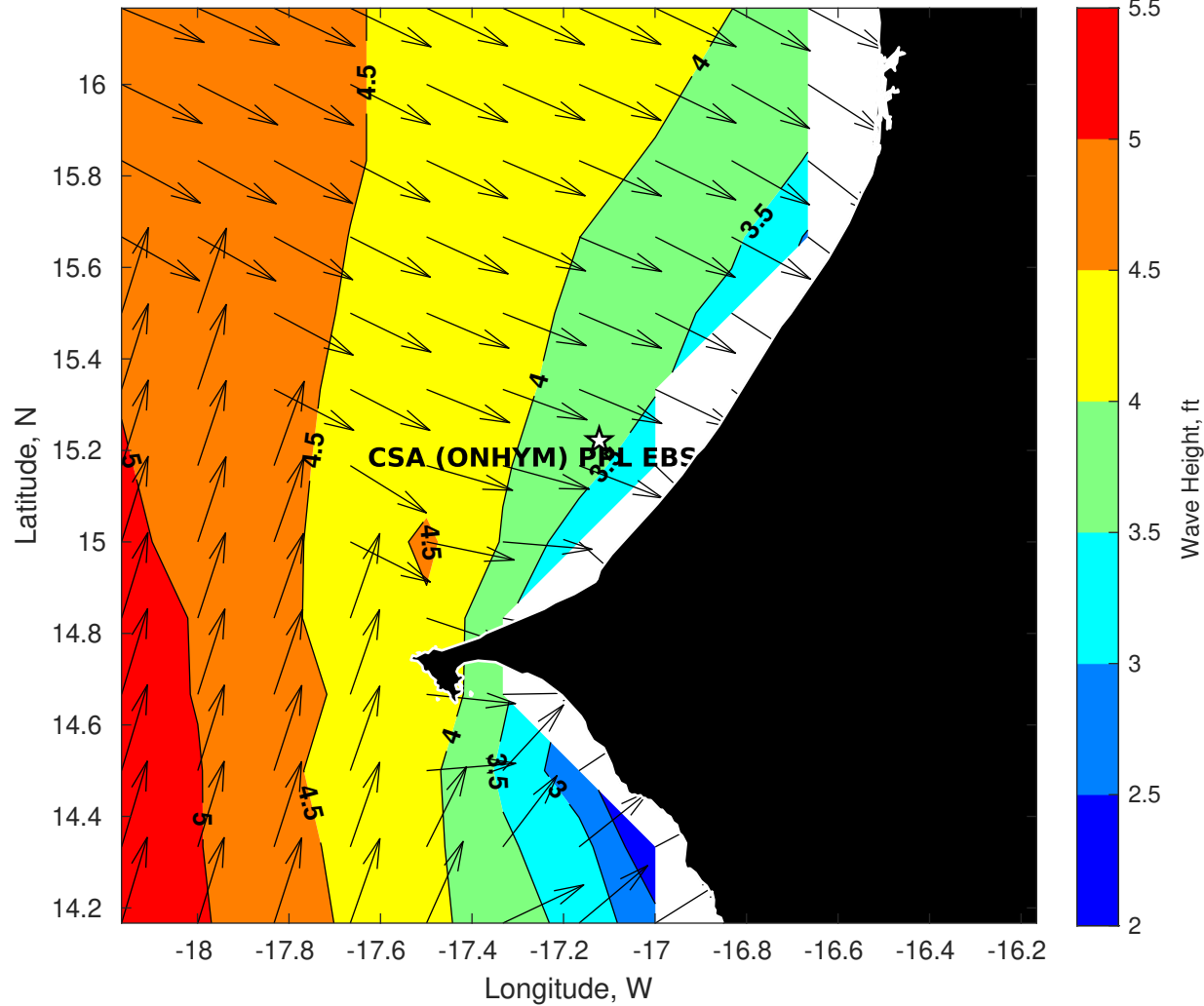
Wave Height (ft) for CSA (ONHYM) PPL EBS - Senegal at 20-Aug-2025 09:00:00
