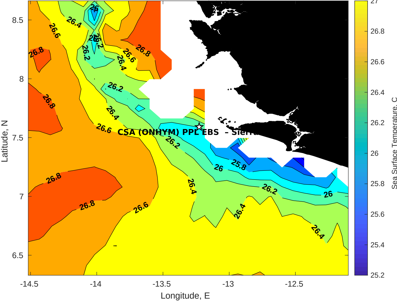
SST for CSA (ONHYM) PPL EBS - Sierra Leone at 19-Aug-2025 00:00:00
