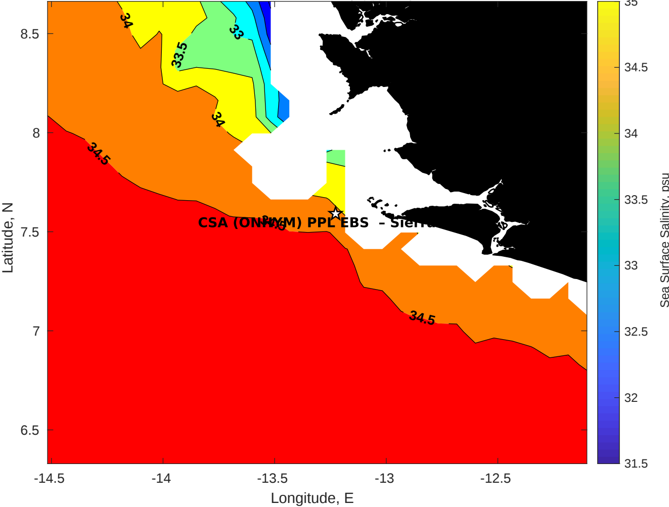
Surface Salinity for CSA (ONHYM) PPL EBS - Sierra Leone at 19-Aug-2025 00:00:00
