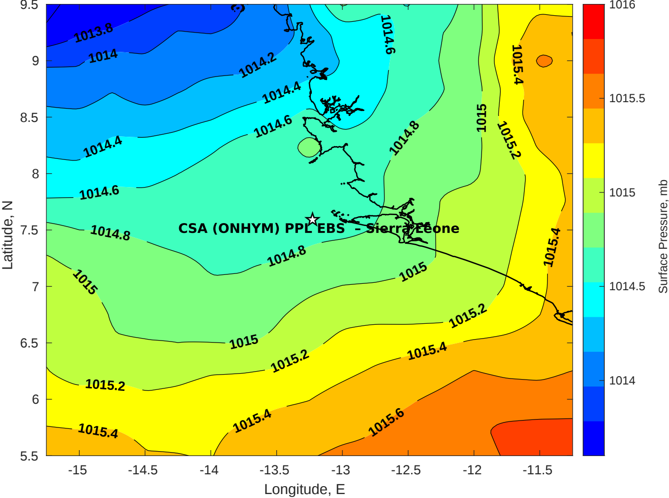
Surface Pressure (mb) for CSA (ONHYM) PPL EBS - Sierra Leone at 21-Aug-2025 00:00:00
