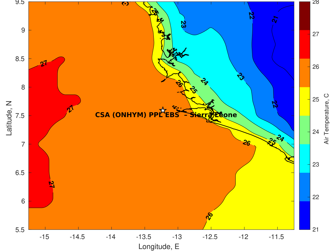
Air Temperature (C) for CSA (ONHYM) PPL EBS - Sierra Leone at 20-Aug-2025
