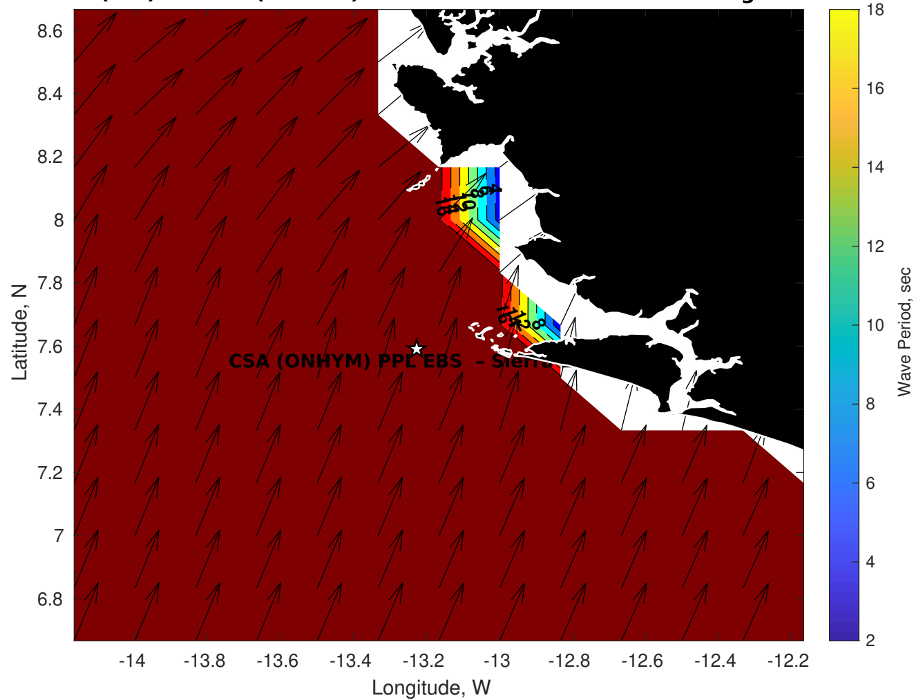
Wave Period (sec) for CSA (ONHYM) PPL EBS - Sierra Leone at 20-Aug-2025 09:00:00
