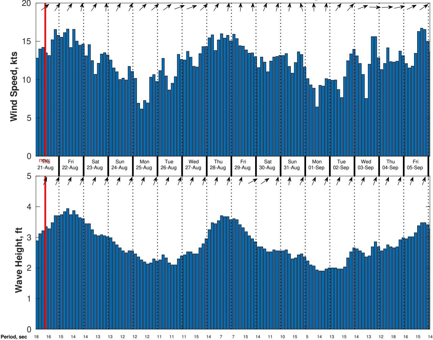
Wind & Wave Forecast for CSA (ONHYM) PPL EBS - Sierra Leone from 20-Aug-2025 01:00:00 to 05-Sep-2025 01:00:00
