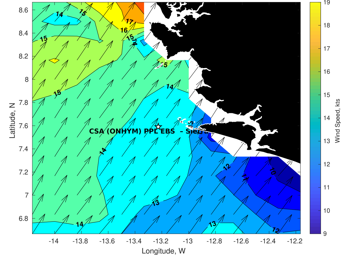
Winds (kts) for CSA (ONHYM) PPL EBS - Sierra Leone at 20-Aug-2025 09:00:00
