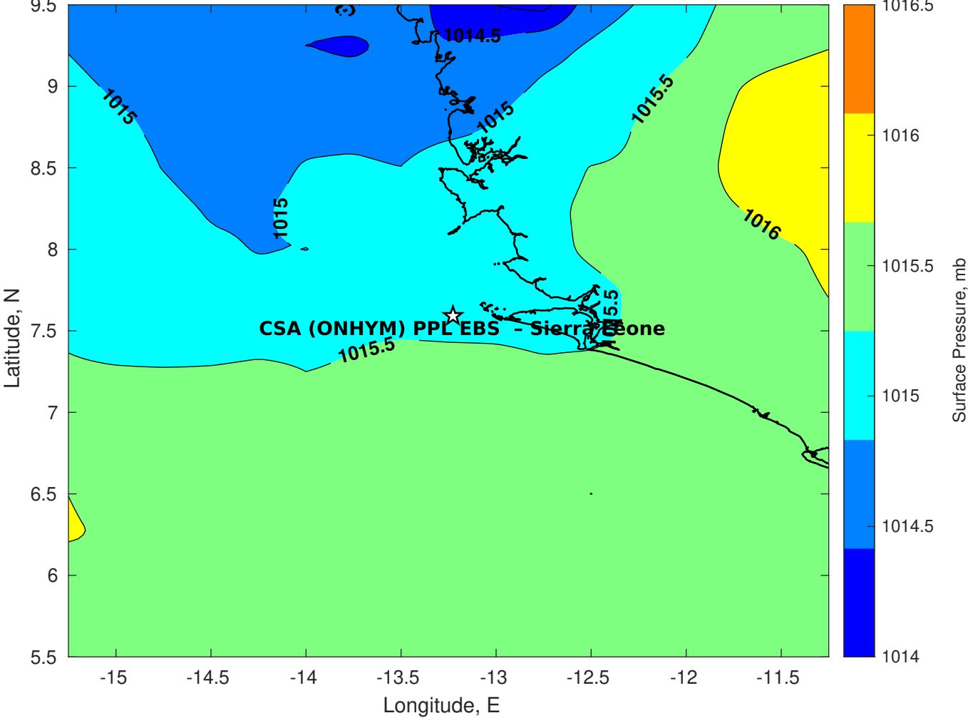
Surface Pressure (mb) for CSA (ONHYM) PPL EBS - Sierra Leone at 20-Aug-2025 00:00:00
