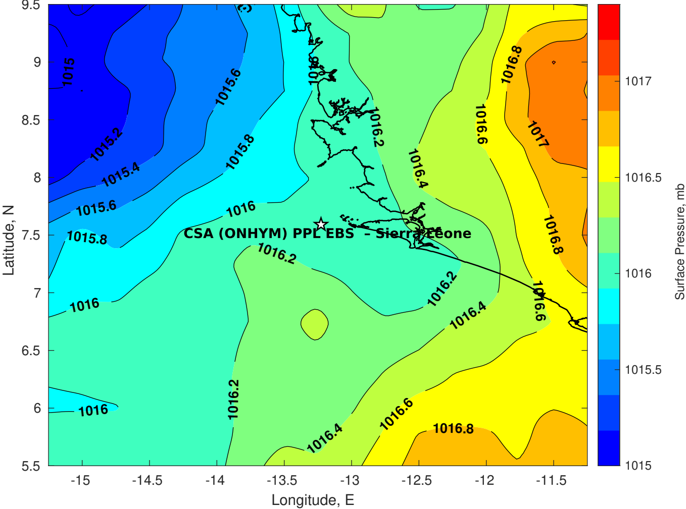
Surface Pressure (mb) for CSA (ONHYM) PPL EBS - Sierra Leone at 22-Aug-2025 00:00:00
