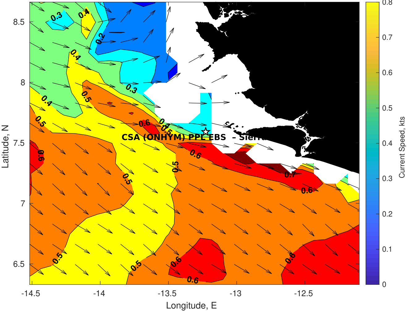
Surface Currents for CSA (ONHYM) PPL EBS - Sierra Leone at 19-Aug-2025 00:00:00
