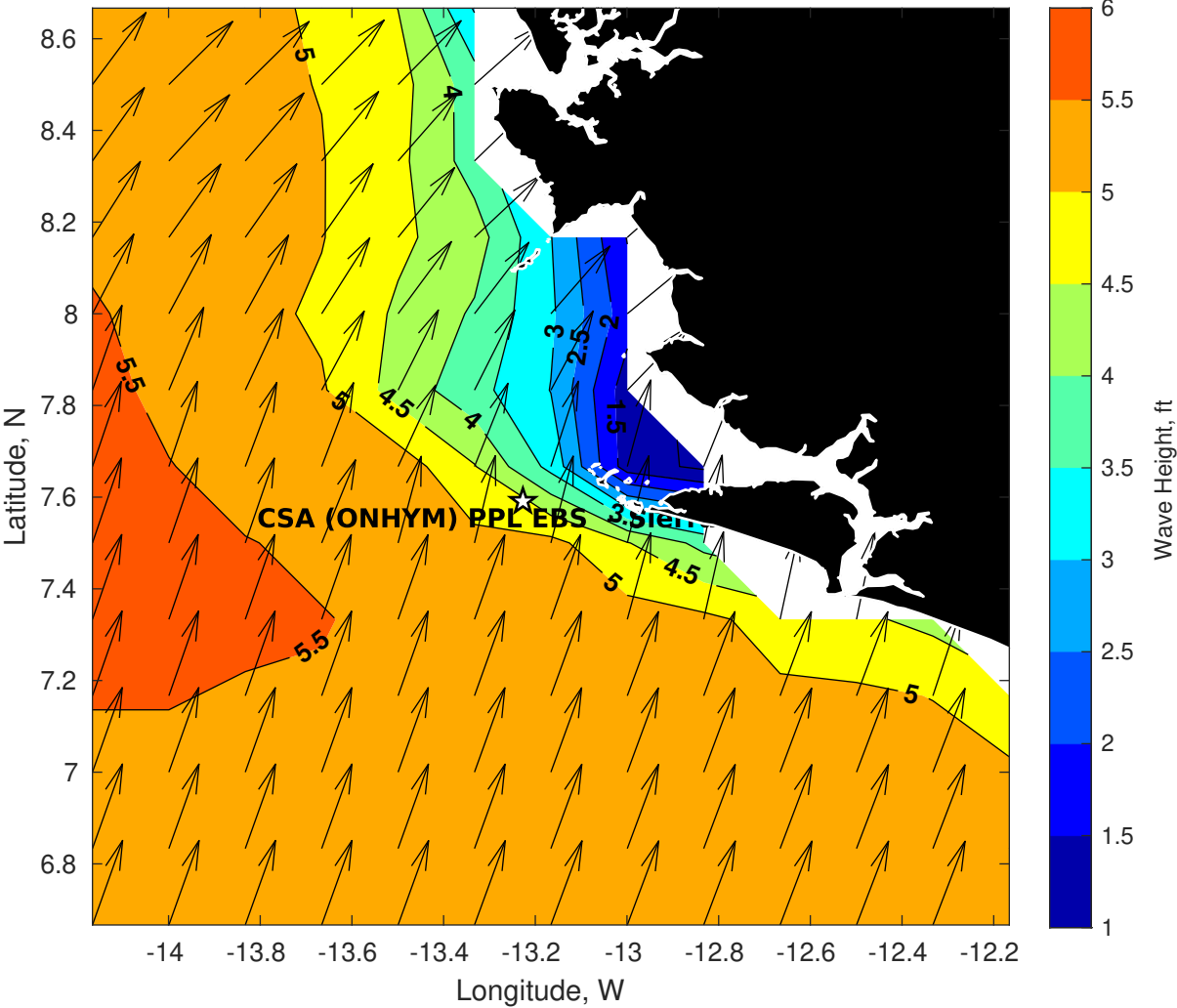
Wave Height (ft) for CSA (ONHYM) PPL EBS - Sierra Leone at 20-Aug-2025 09:00:00
