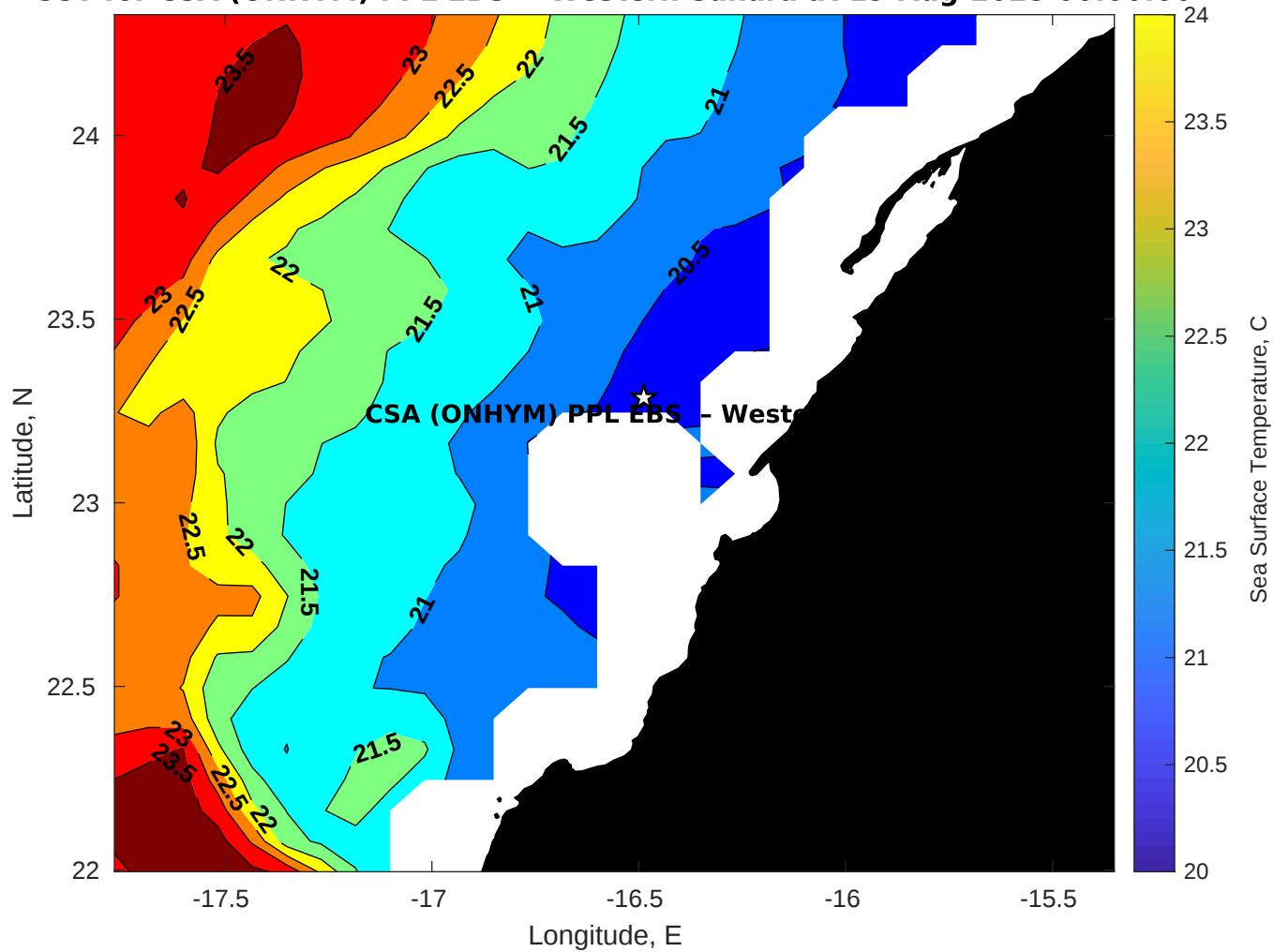
SST for CSA (ONHYM) PPL EBS - Western Sahara at 19-Aug-2025 00:00:00
