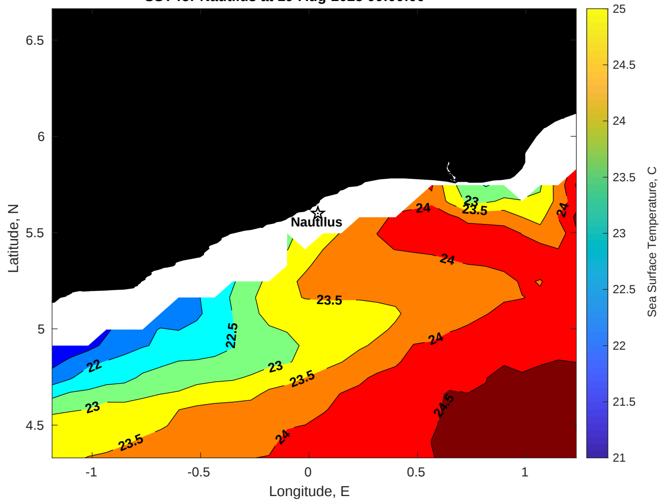
SST for Nautilus at 19-Aug-2025 00:00:00
