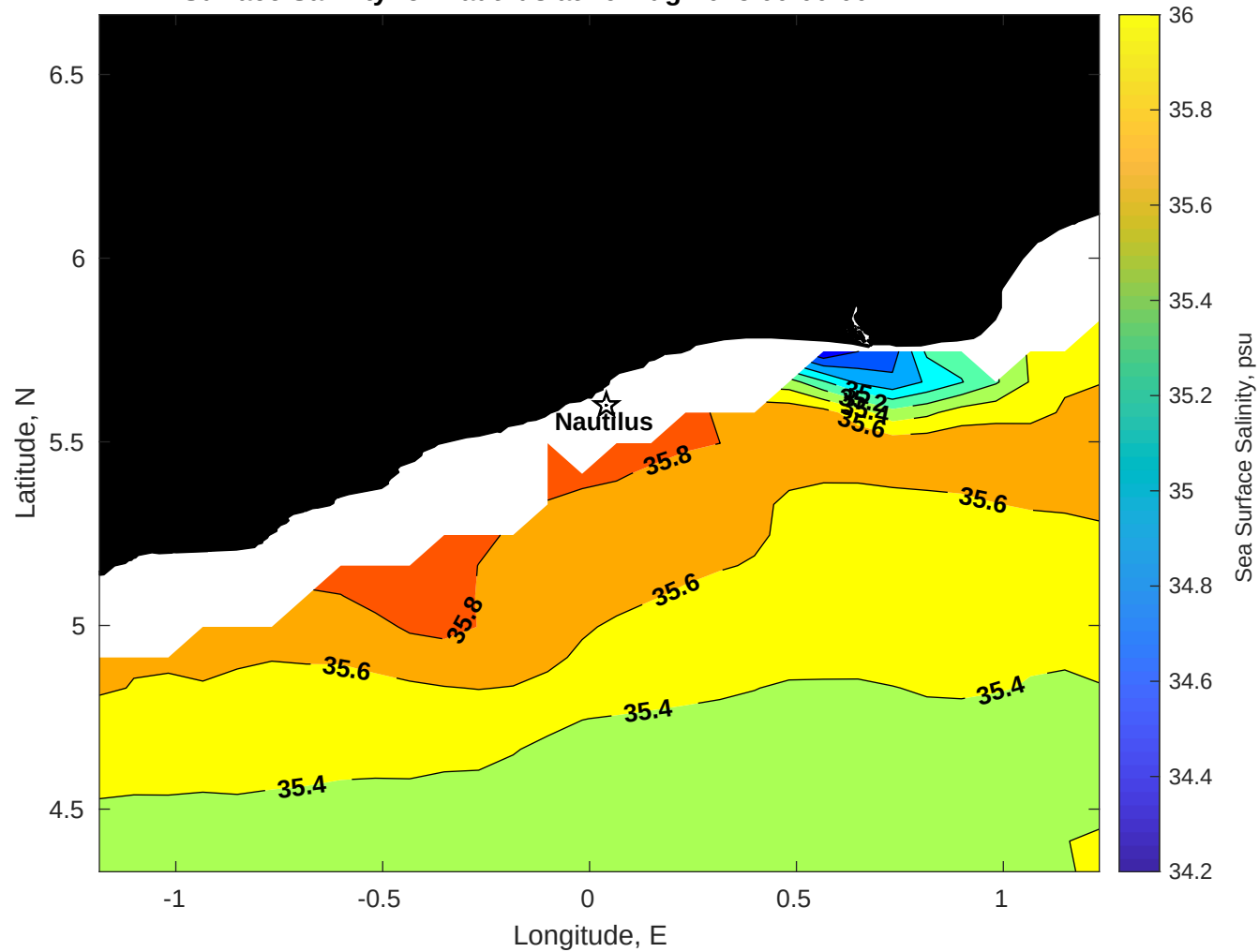
Surface Salinity for Nautilus at 19-Aug-2025 00:00:00
