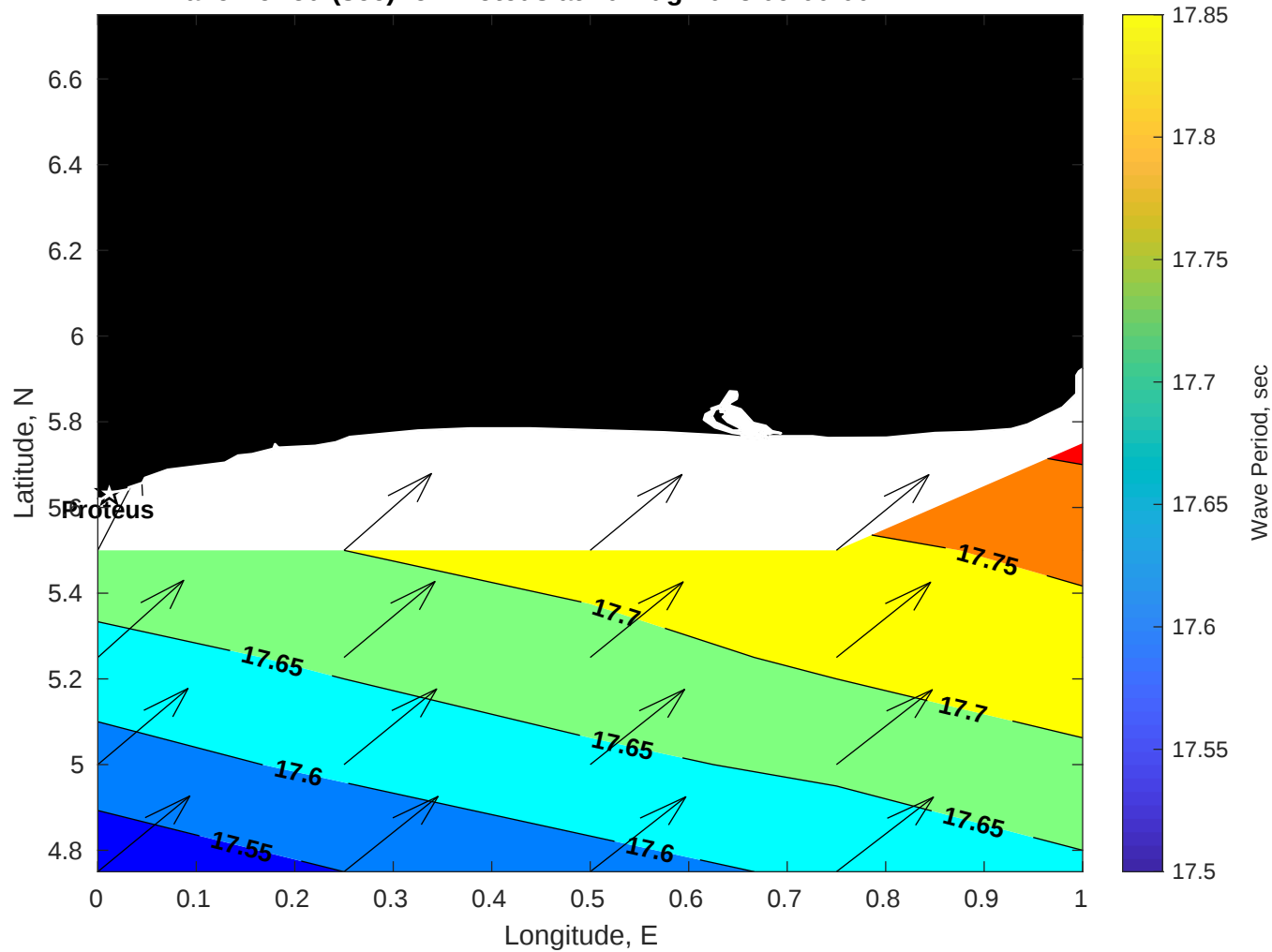
Wave Period (sec) for Proteus at 20-Aug-2025 09:00:00
