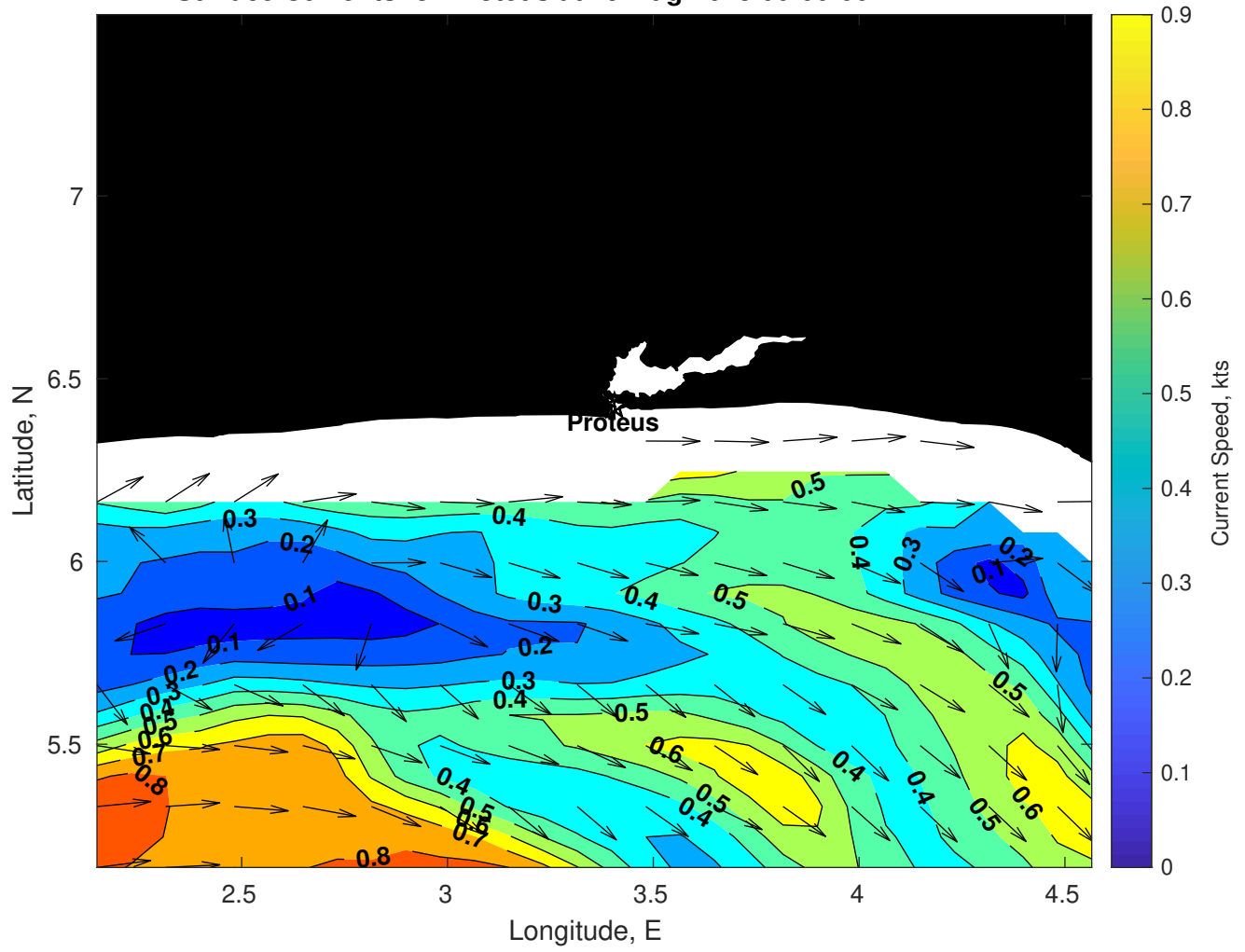
Surface Currents for Proteus at 19-Aug-2025 00:00:00
