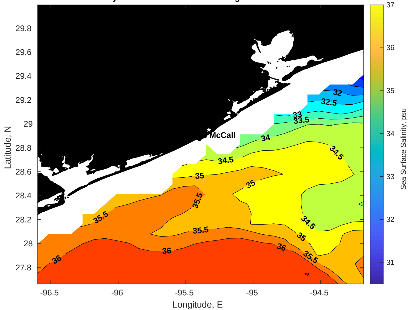
Surface Salinity for Brooks McCall at 20-Aug-2025 00:00:00
