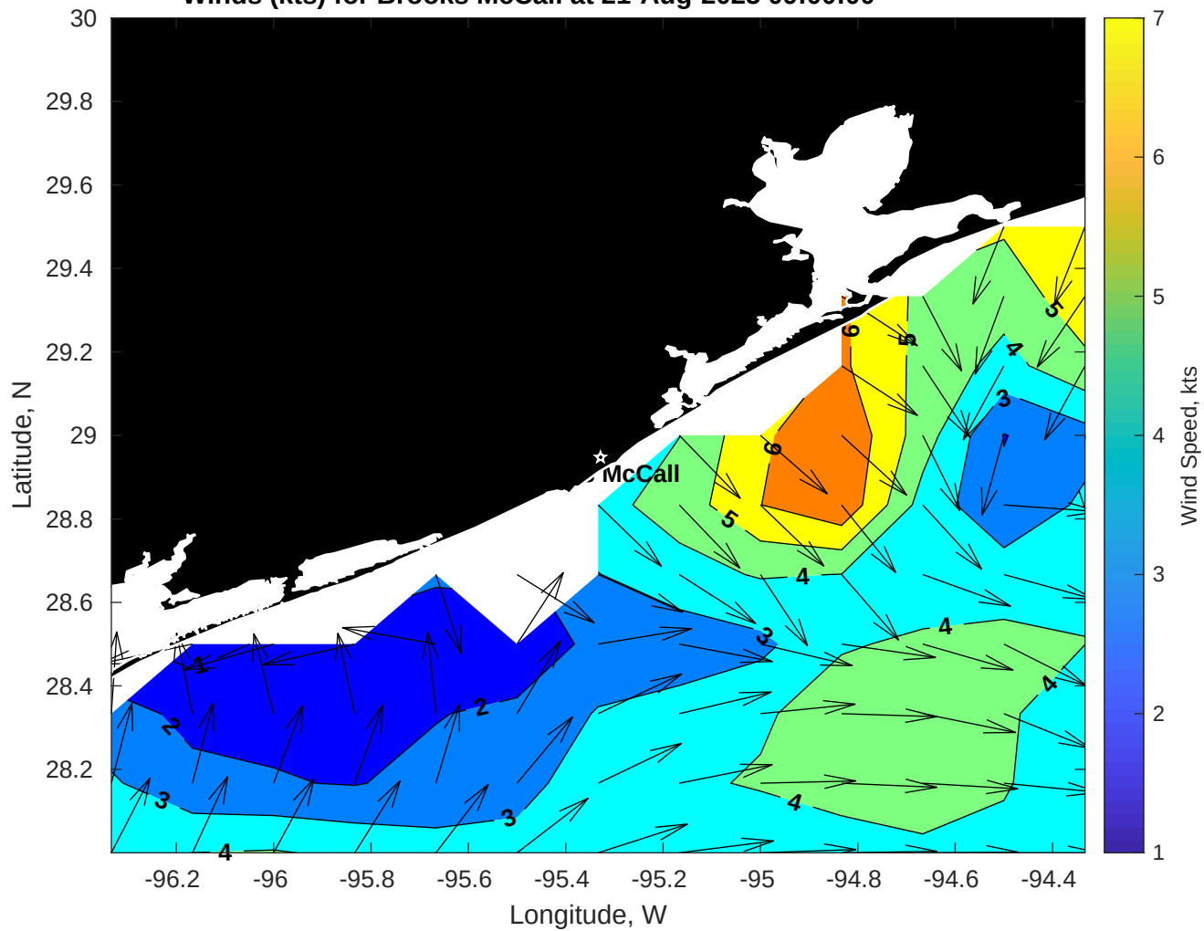
Winds (kts) for Brooks McCall at 21-Aug-2025 09:00:00
