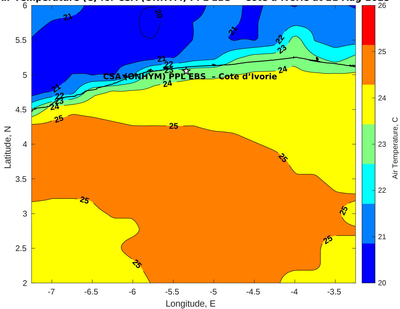
Air Temperature (C) for CSA (ONHYM) PPL EBS - Cote d'Ivoire at 21-Aug-2025
