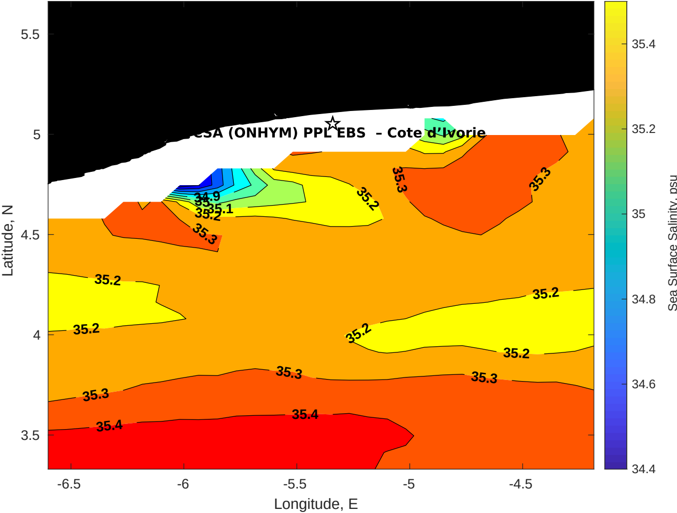
Surface Salinity for CSA (ONHYM) PPL EBS - Cote d'Ivoire at 20-Aug-2025 00:00:00
