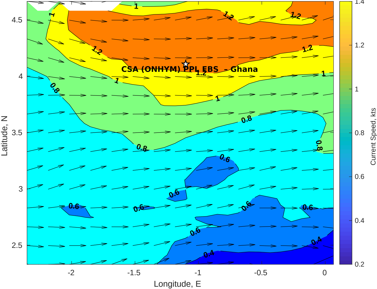
Surface Currents for CSA (ONHYM) PPL EBS - Ghana at 20-Aug-2025 00:00:00
