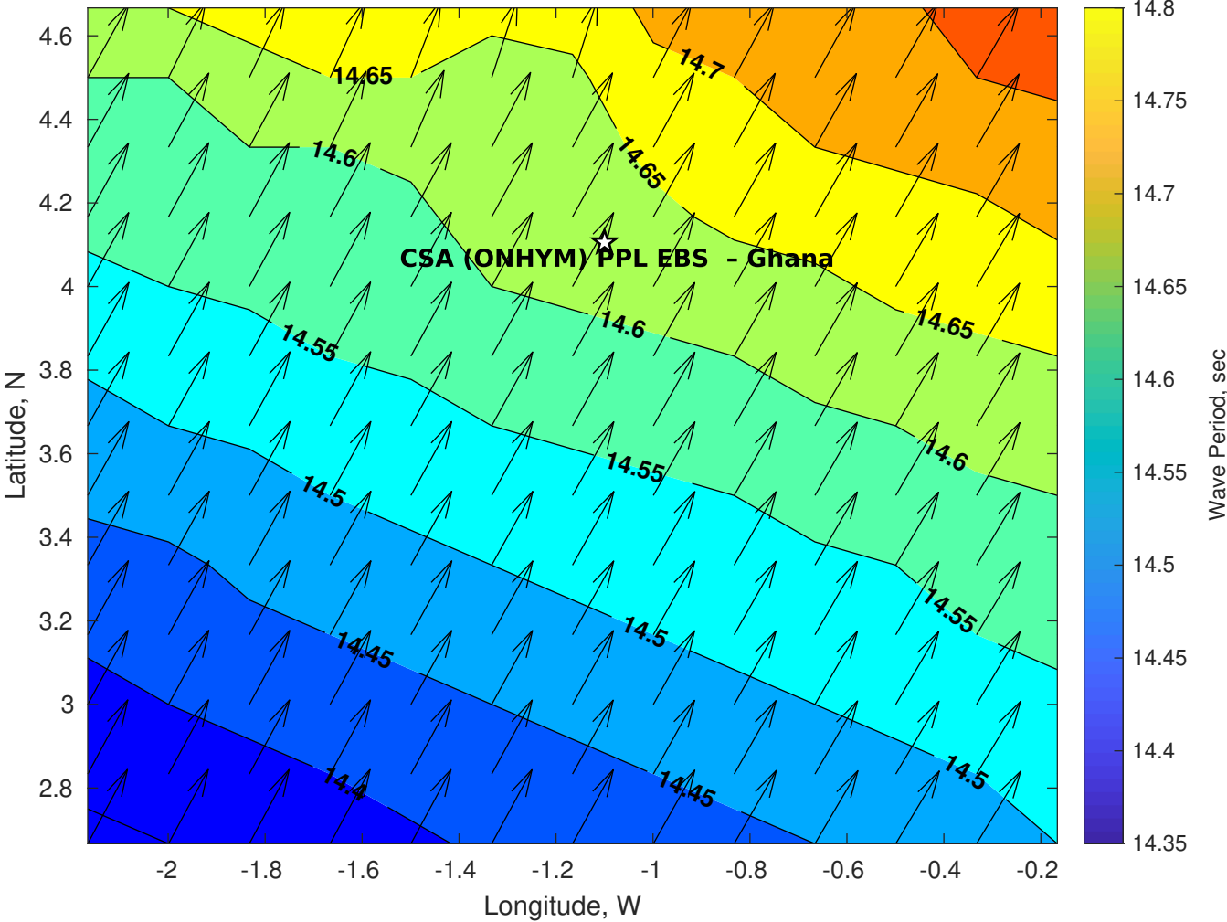
Wave Period (sec) for CSA (ONHYM) PPL EBS - Ghana at 21-Aug-2025 09:00:00
