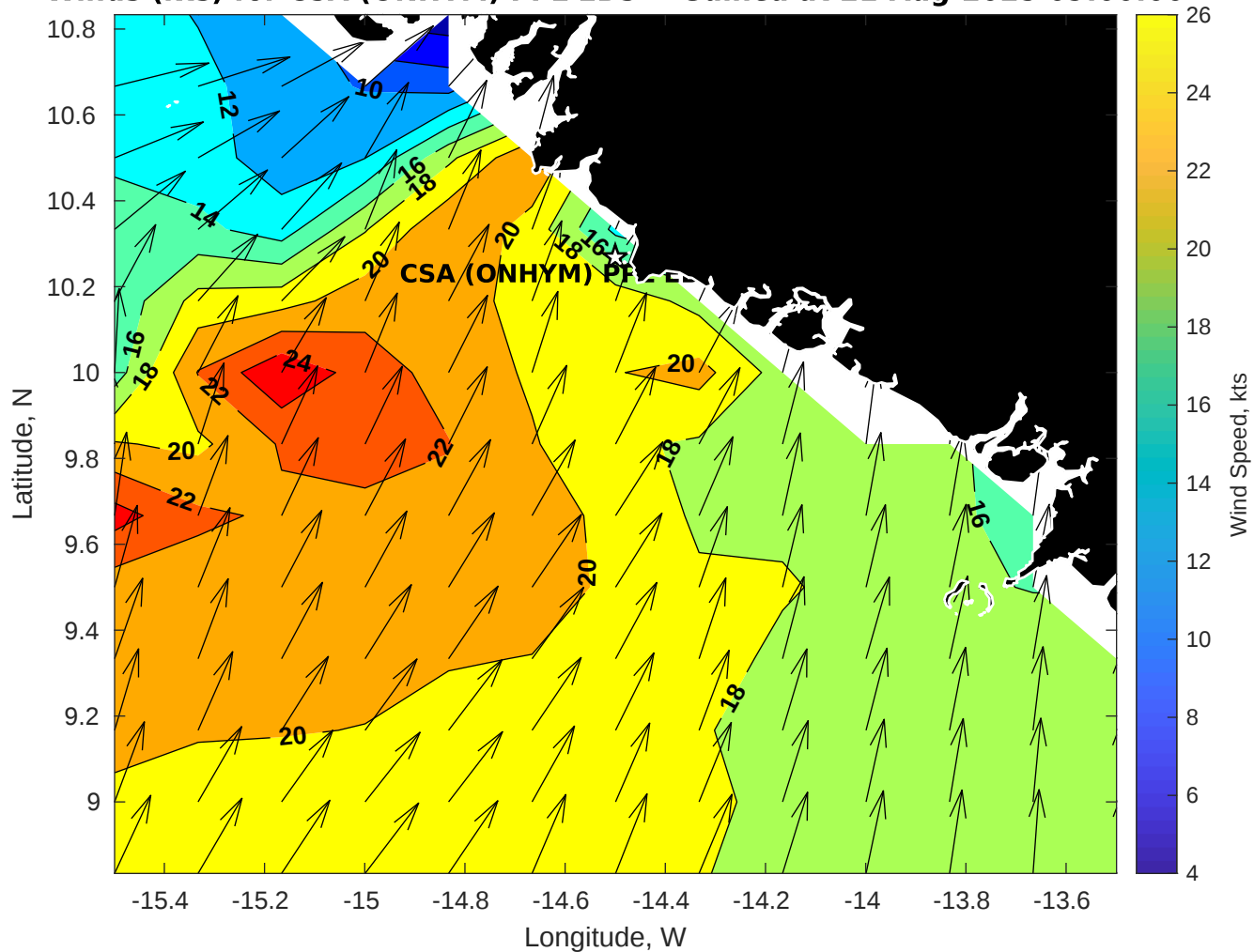
Winds (kts) for CSA (ONHYM) PPL EBS - Guinea at 21-Aug-2025 09:00:00
