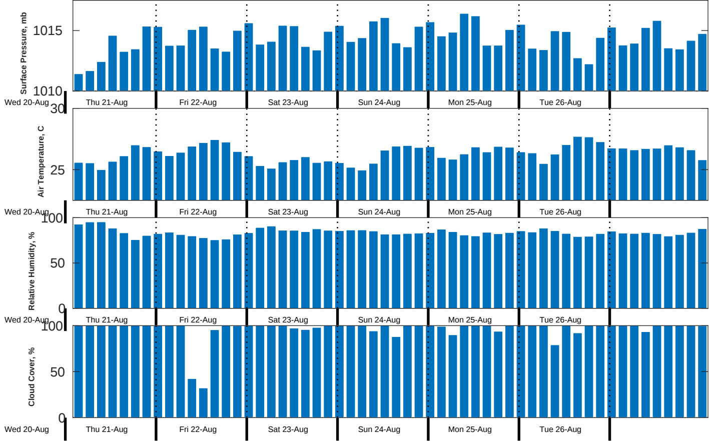
Met Forecast for CSA (ONHYM) PPL EBS - Guinea from 21-Aug-2025 00:00:00 to 28-Aug-2025 00:00:00
