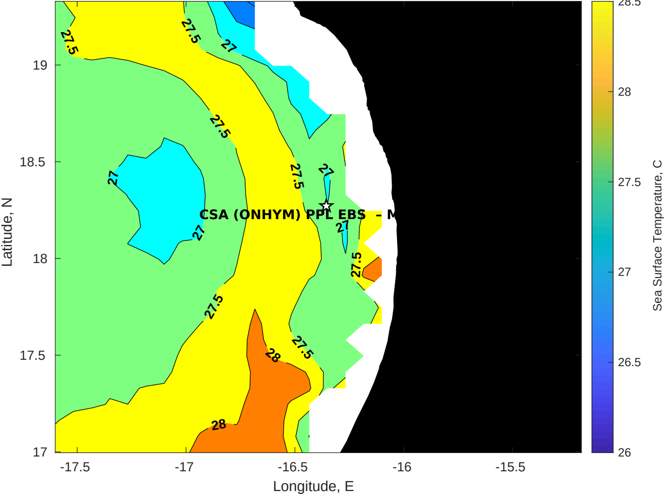
SST for CSA (ONHYM) PPL EBS - Mauritania at 20-Aug-2025 00:00:00
