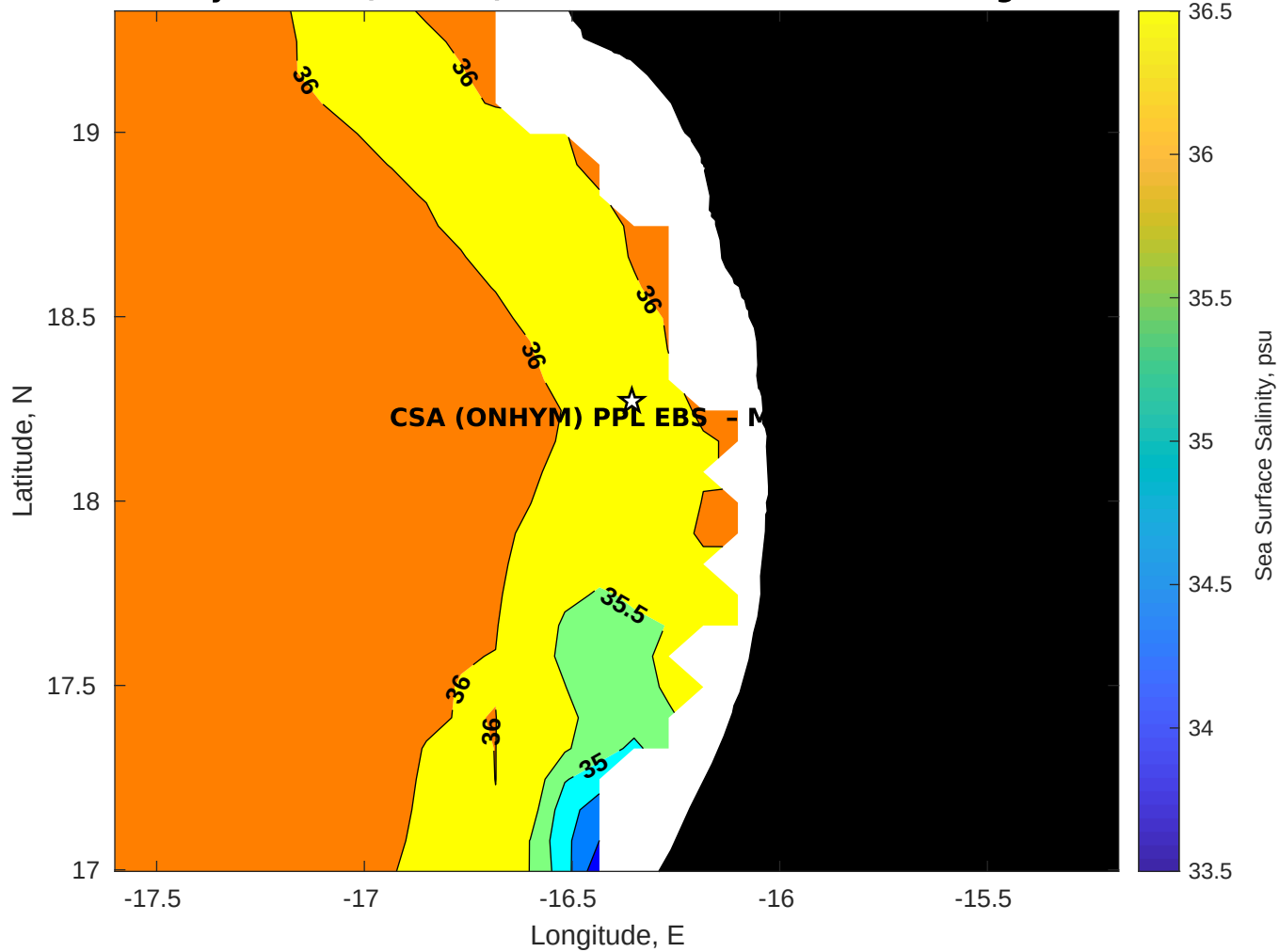
Surface Salinity for CSA (ONHYM) PPL EBS - Mauritania at 20-Aug-2025 00:00:00
